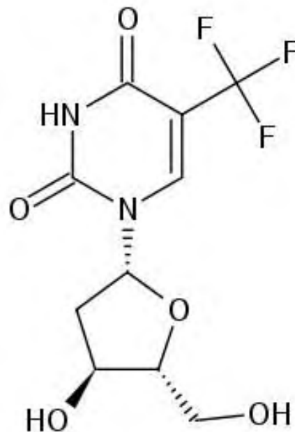
Trifluridine trifluorothymidine (TFT)
