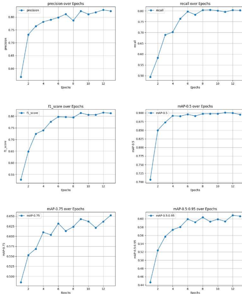
Figure 4.41: Plots per epoch for SSD with VGG16 (RGB dataset)
