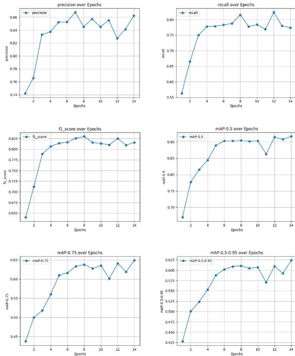
Figure 4.47: Plots per epoch for EfficientDet D1 (Thermal dataset)
