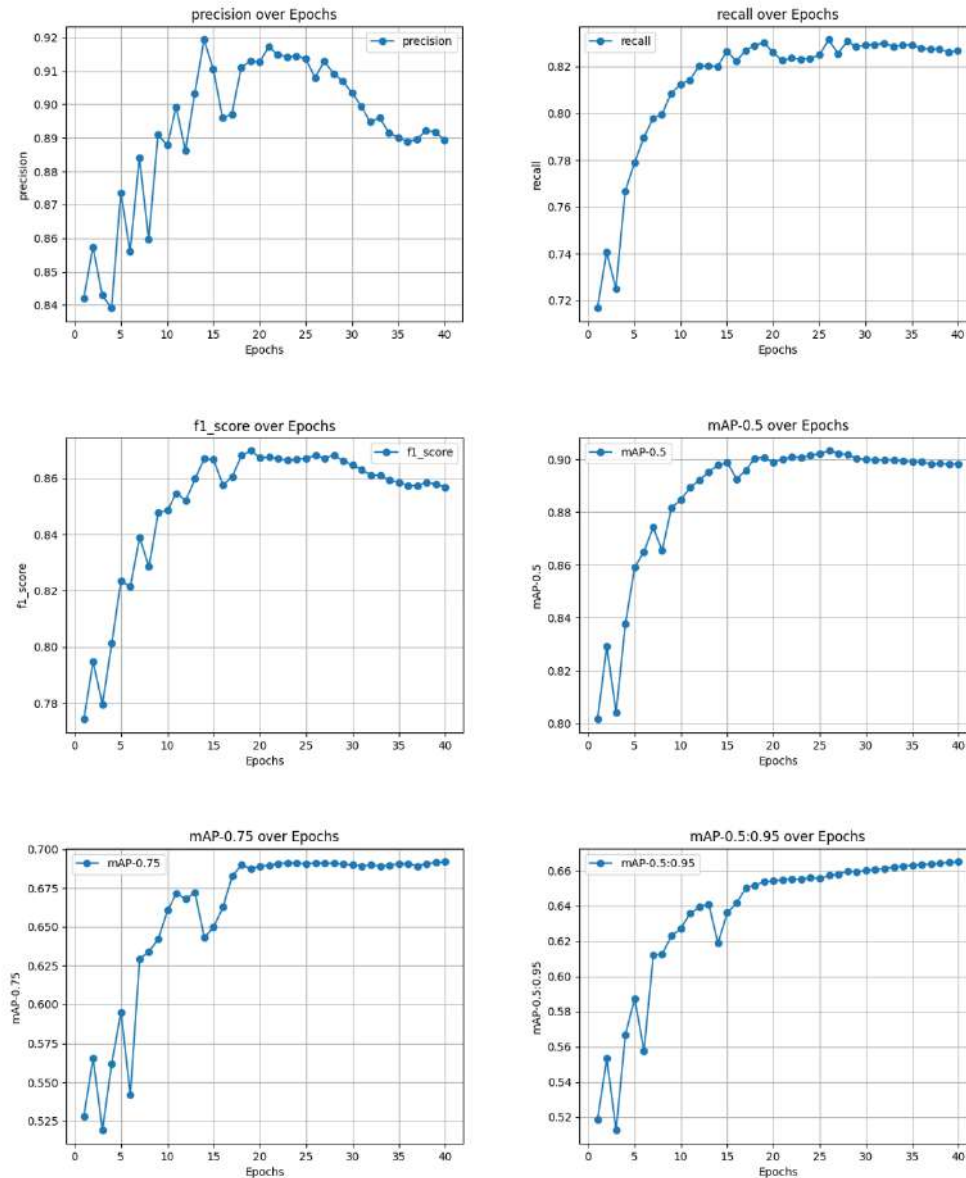
Figure 4.33: Plots per epoch for YOLOv8s (RGB dataset)
