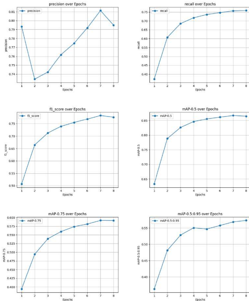
Figure 4.37: Plots per epoch for Faster R-CNN with MobileNetV3 (RGB dataset)
