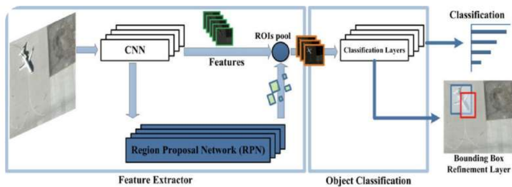
Figure 4.26: Faster R-CNN architecture [60]
