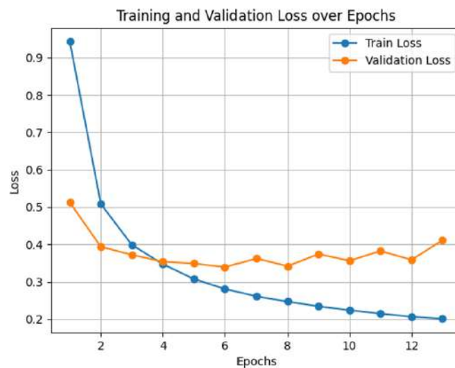
Figure 4.44: Training and validation loss curves for EfficientDet D1 (RGB dataset)
