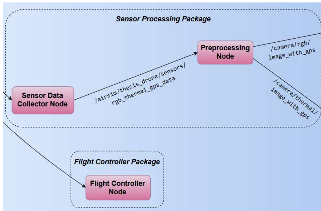
Figure 5.22: ROS 2 architecture part 1
