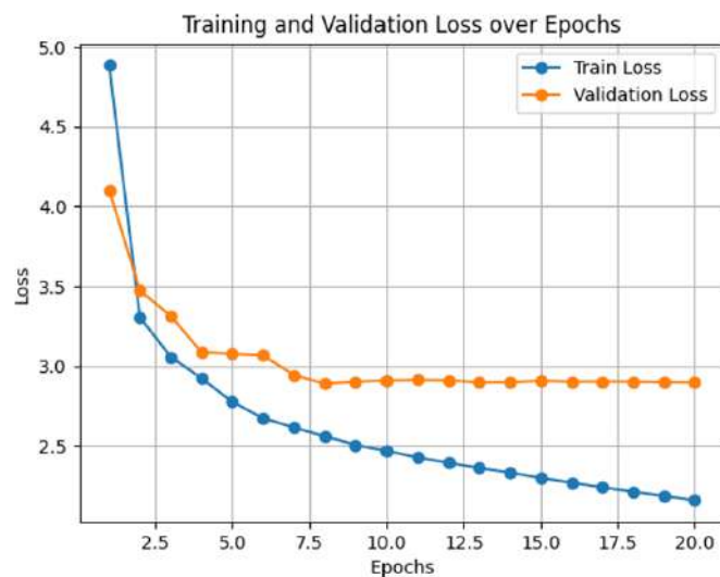
Figure 4.34: Training and validation loss curves for YOLOv8s (Thermal dataset)
