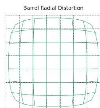
Figure 5.4: Negative (barrel) distortion [70]
