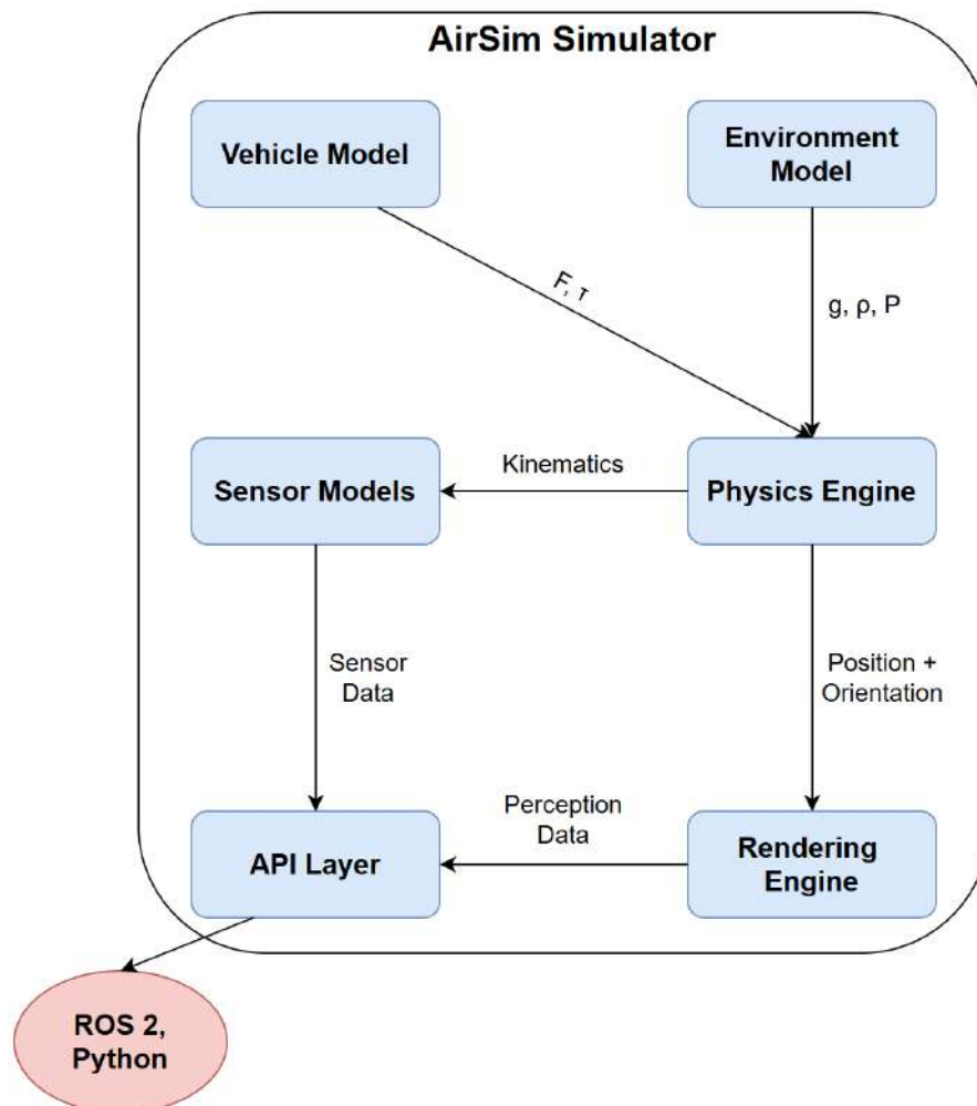
Figure 6.1: AirSim Internal Simulation Architecture
