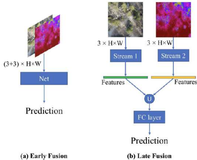
Figure 3.1: Fusion techniques [22]
