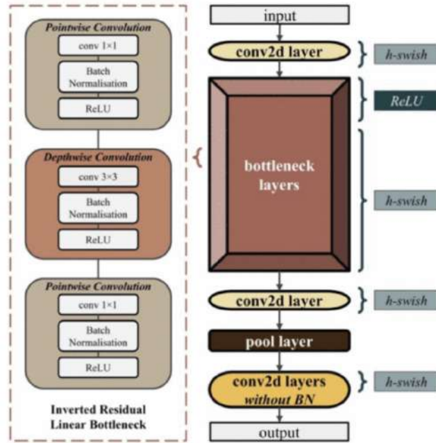
Figure 4.25: MobileNetV3 architecture [58]
