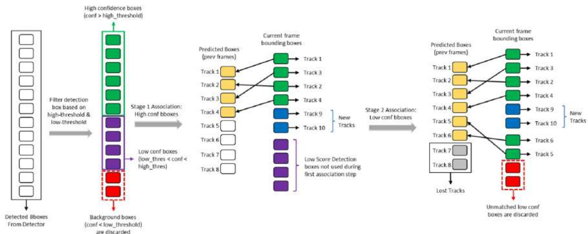
Figure 5.7: ByteTrack algorithm [71]
