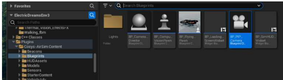
Figure 6.19: BP_PIP_Camera blueprint
