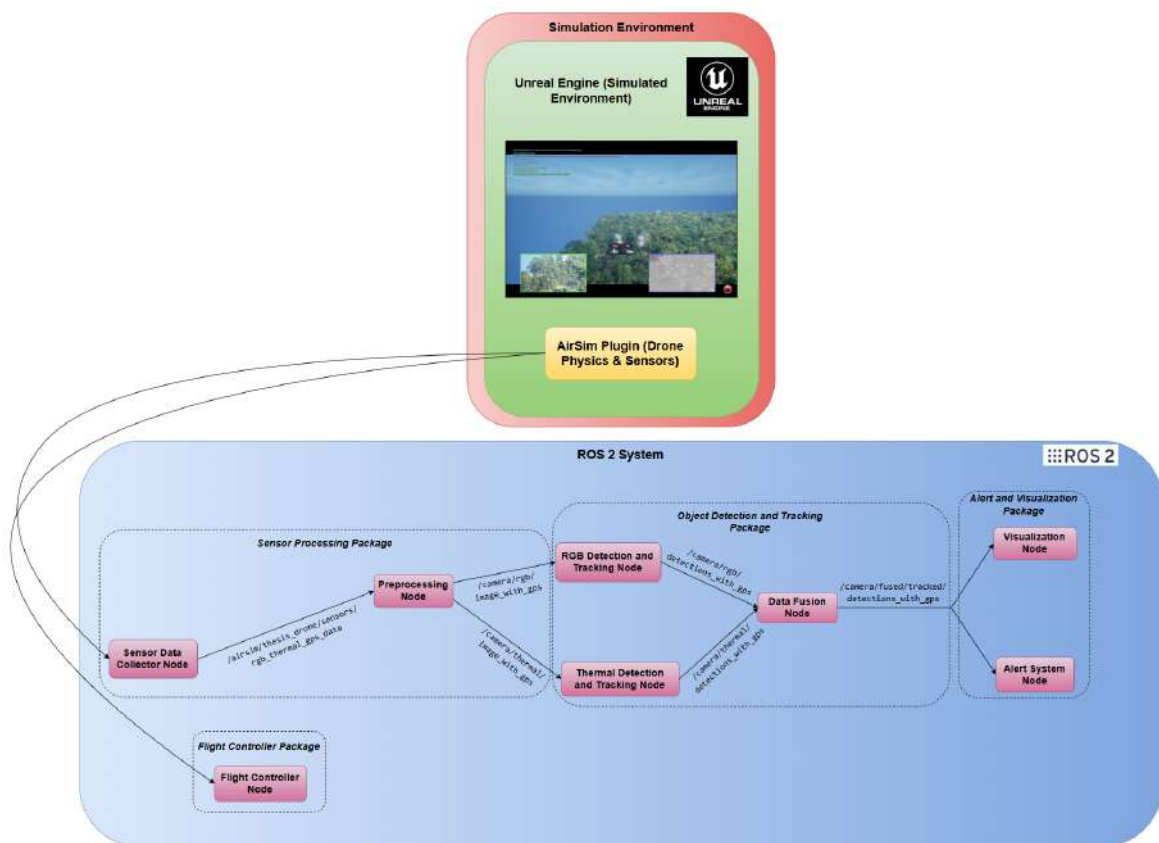
Figure 5.21: ROS 2 architecture
