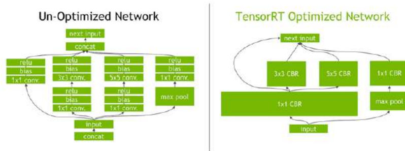
Figure 4.58: Layer and tensor fusion [68]
