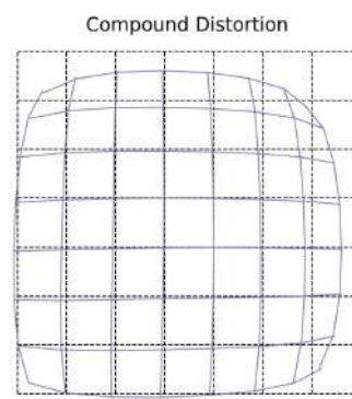
Figure 5.6: Barrel + pincushion + tangential [70]
