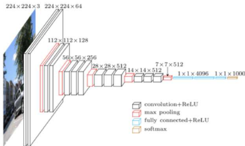
Figure 4.27: VGG16 architecture [62]
