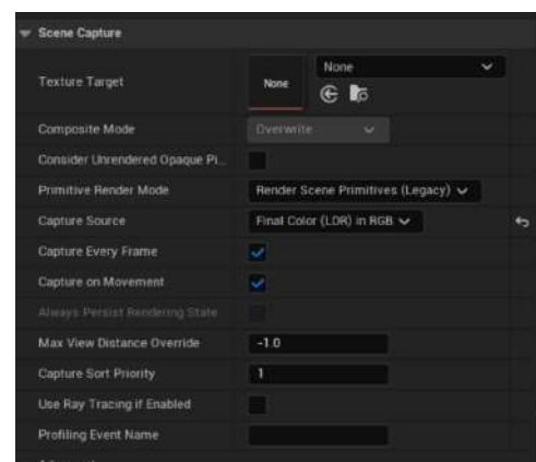
Figure 6.22: Scene capture settings part 1
