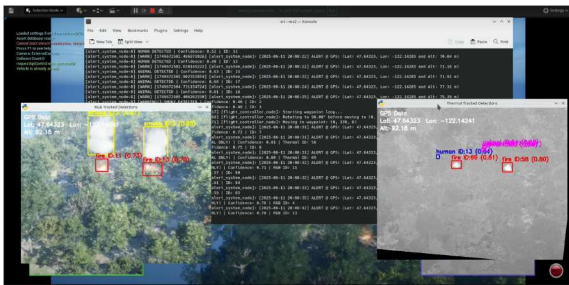
Figure 7.1: Combined RGB and Thermal/IR camera feeds with object detection and tracking (1st example)
