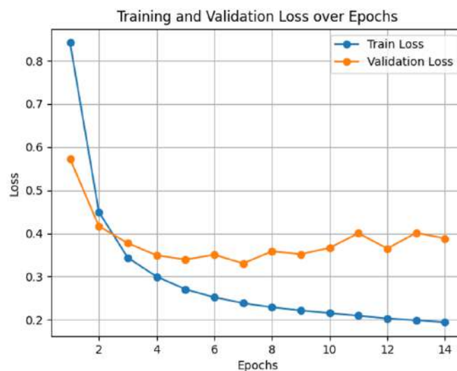
Figure 4.46: Training and validation loss curves for EfficientDet D1 (Thermal dataset)
