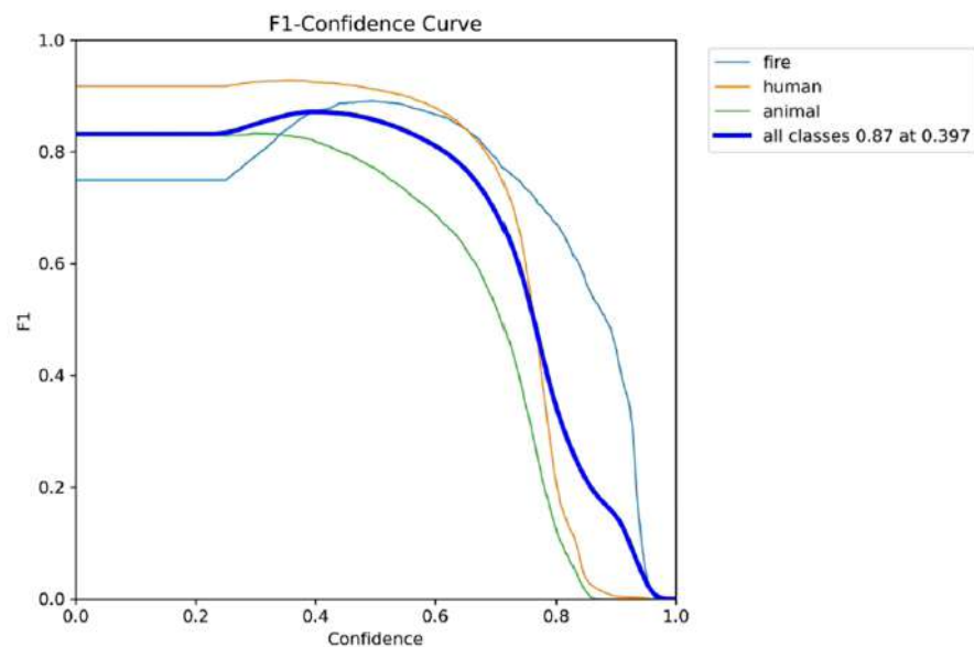
Figure 4.51: F1-Confidence curve on the Thermal valid dataset
