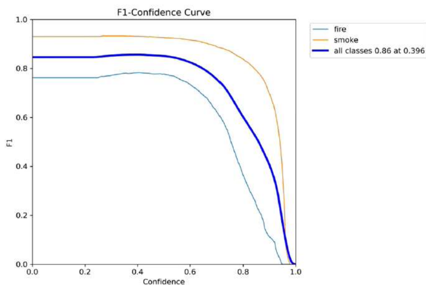
Figure 4.48: F1-Confidence curve on the RGB valid dataset
