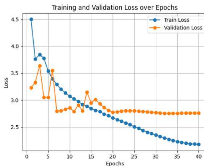
Figure 4.32: Training and validation loss curves for YOLOv8s (RGB dataset)
