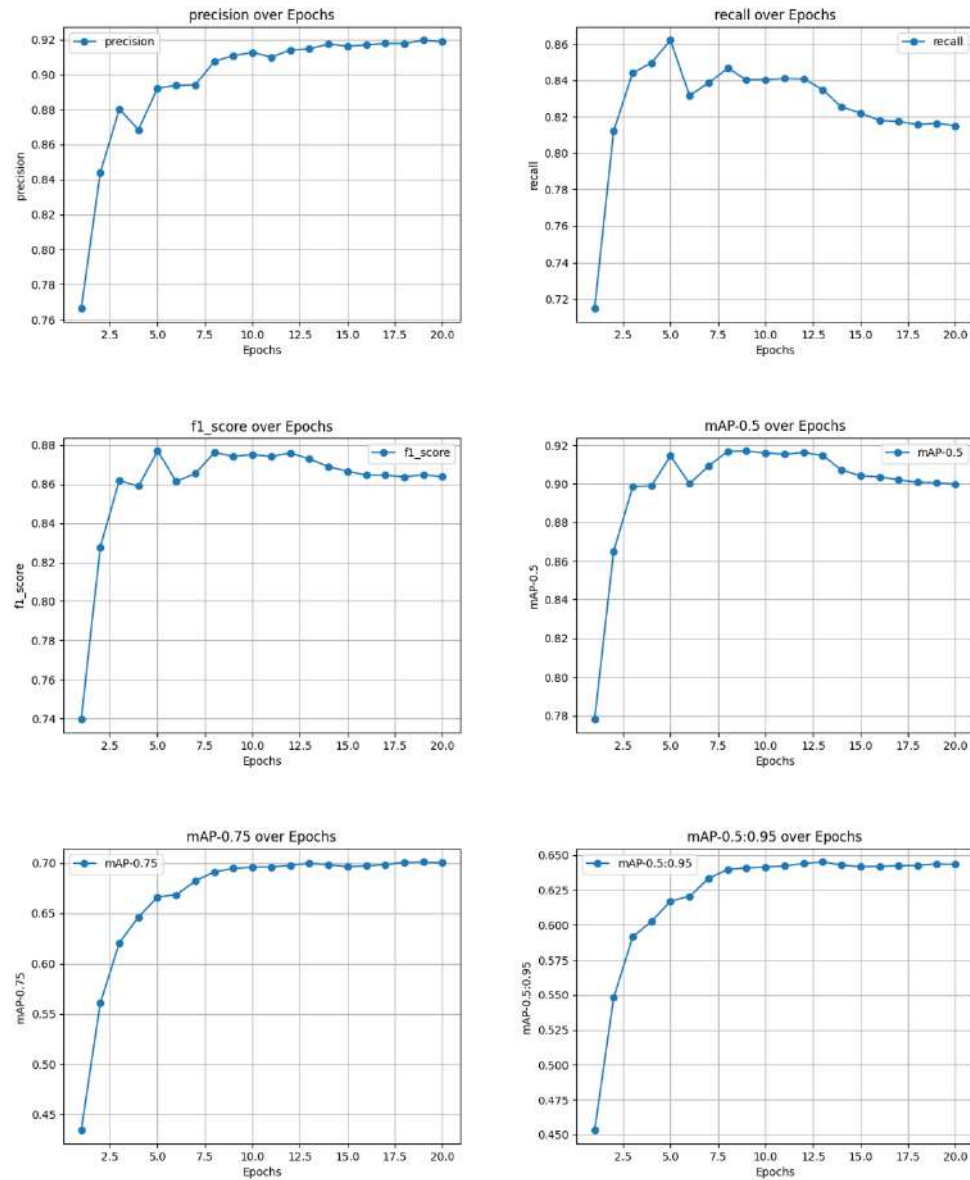
Figure 4.35: Plots per epoch for YOLOv8s (Thermal dataset)
