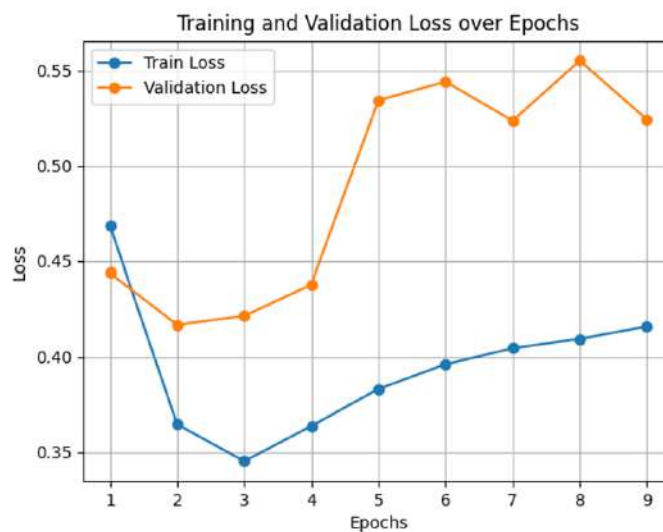
Figure 4.38: Training and validation loss curves for Faster R-CNN with MobileNetV3 (Thermal dataset)
