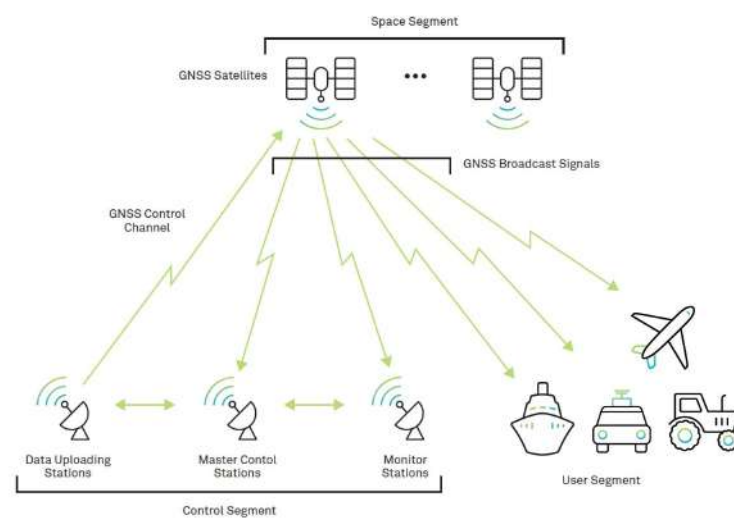
Figure 2.8: GPS structure [17]
