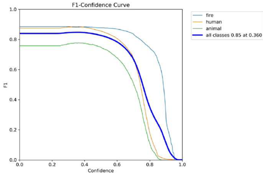
Figure 4.52: F1-Confidence curve on the Thermal test dataset
