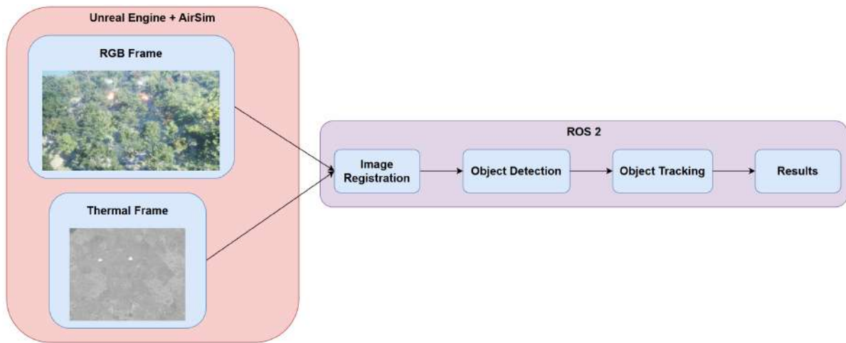
Figure 5.1: System architecture
