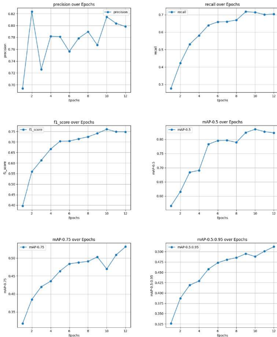
Figure 4.43: Plots per epoch for SSD with VGG16 (Thermal dataset)
