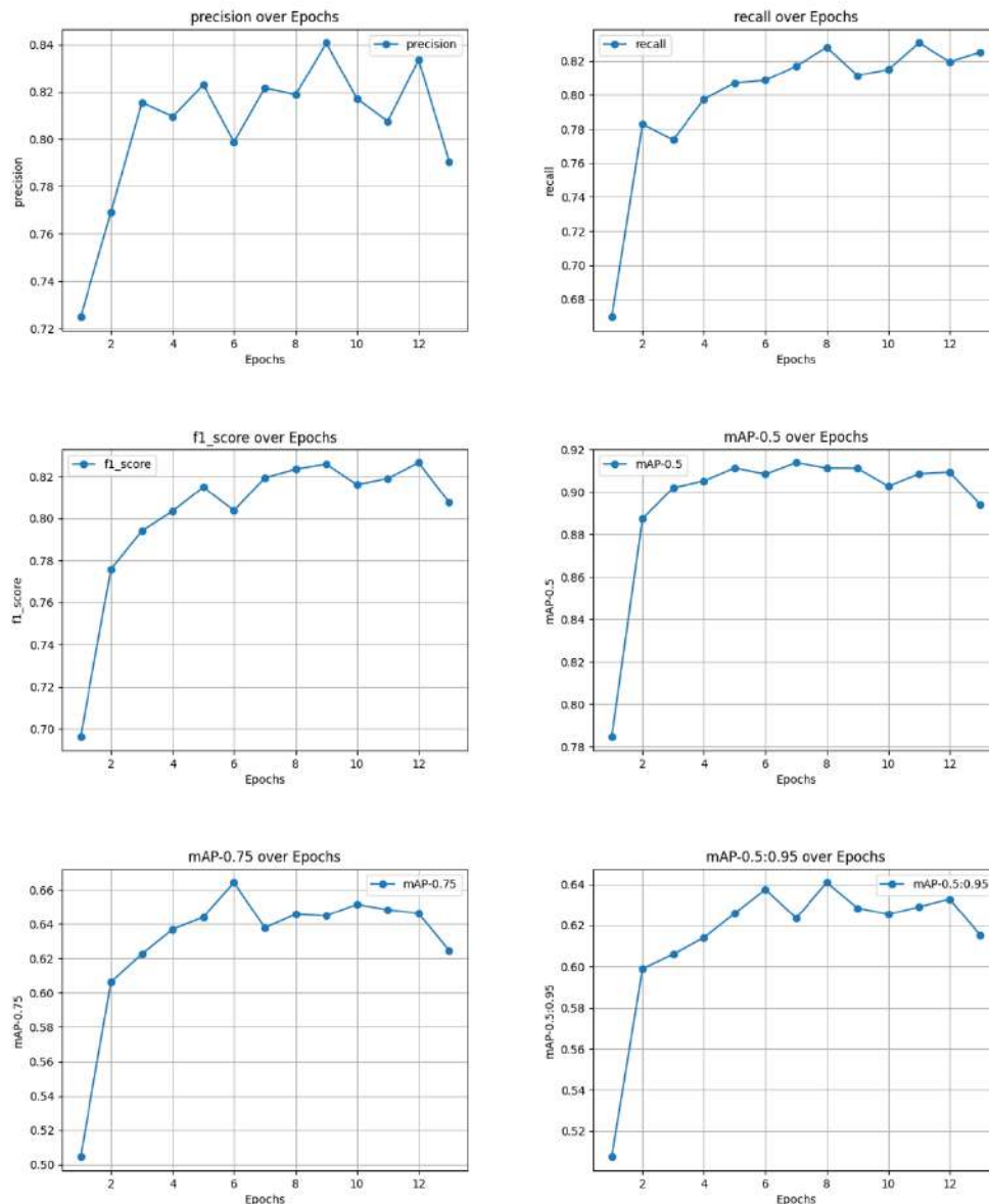
Figure 4.45: Plots per epoch for EfficientDet D1 (RGB dataset)
