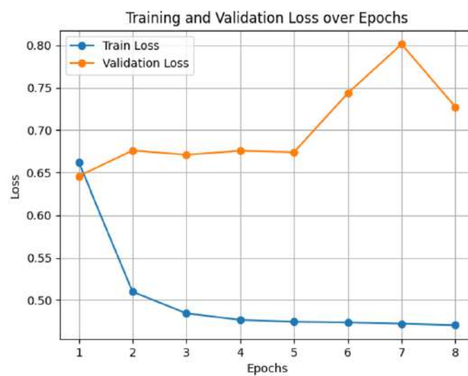
Figure 4.36: Training and validation loss curves for Faster R-CNN with MobileNetV3 (RGB dataset)
