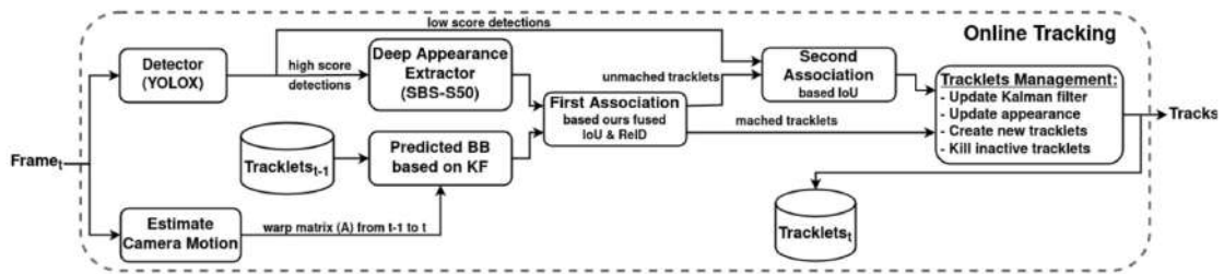
Figure 5.9: BoT-SORT-ReID tracker pipeline [76]
