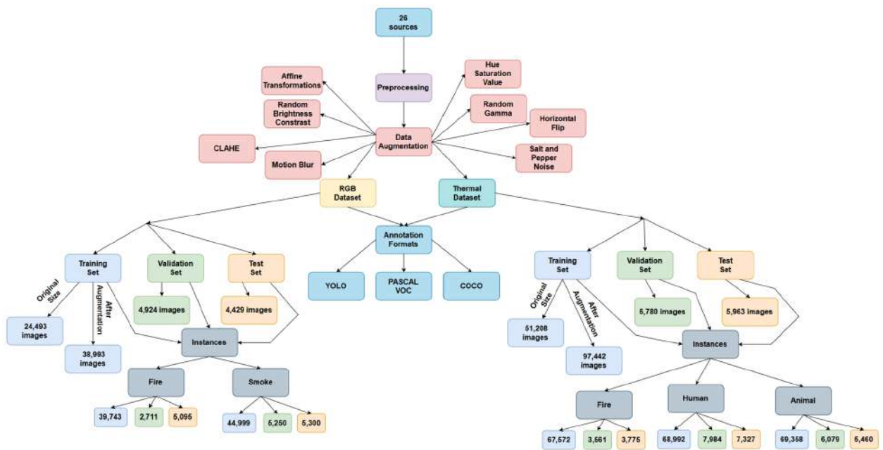
Figure 4.19: Datasets construction and augmentation pipeline
