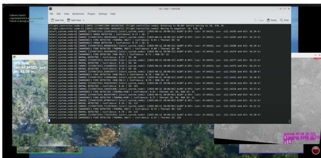
Figure 7.7: Terminal logs showing detection alerts from both domains (2nd example)
