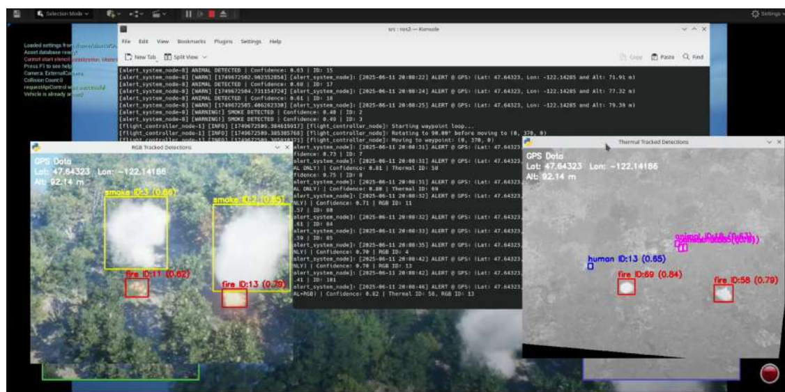
Figure 7.2: Combined RGB and Thermal/IR camera feeds with object detection and tracking (2nd example)
