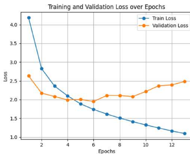
Figure 4.40: Training and validation loss curves for SSD with VGG16 (RGB dataset)
