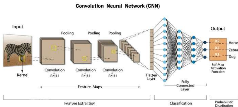
Figure 2.3: Convolutional neural network (CNN) architecture [4]
