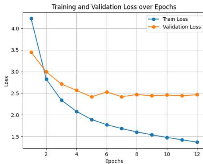
Figure 4.42: Training and validation loss curves for SSD with VGG16 (Thermal dataset)
