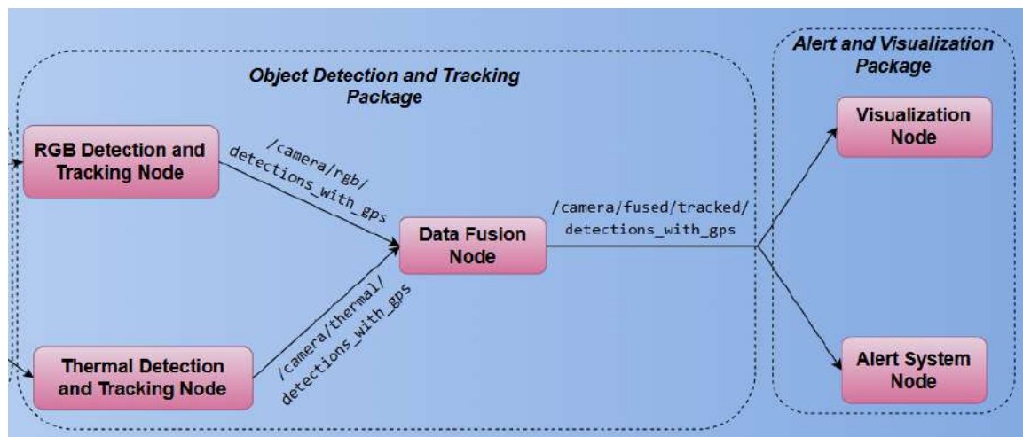
Figure 5.23: ROS 2 architecture part 2
