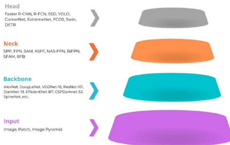
Figure 2.4: Object detection components [5]
