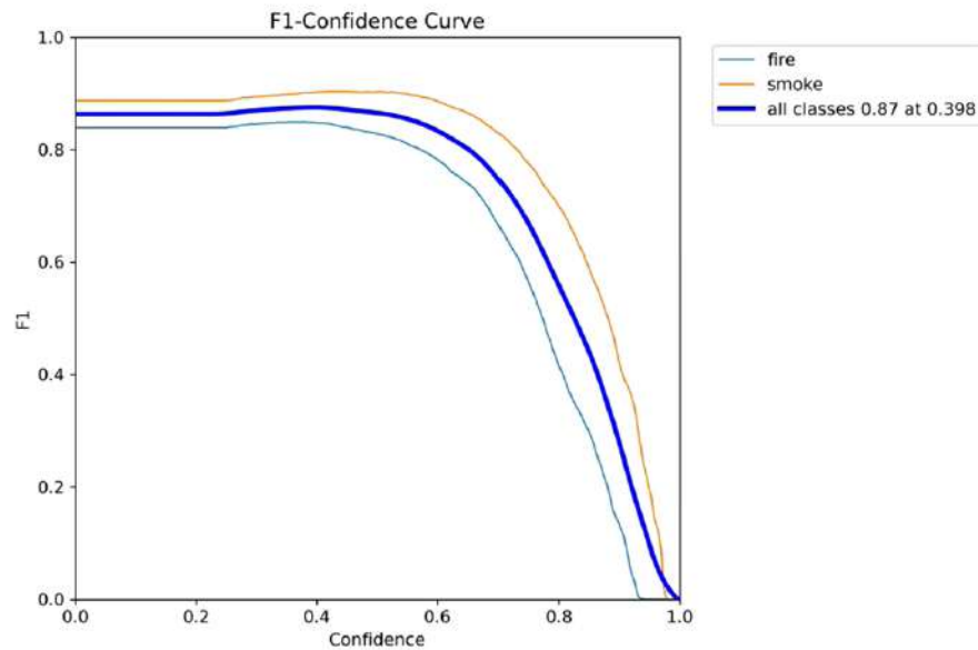
Figure 4.49: F1-Confidence curve on the RGB test dataset
