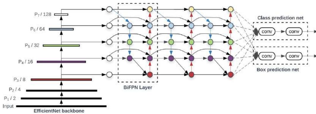
Figure 4.29: EfficientDet architecture [64]
