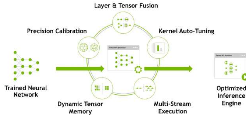
Figure 4.54: TensorRT functionality [68]
