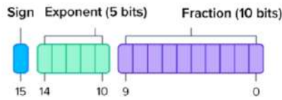
Figure 4.56: FP16 representation [69]
