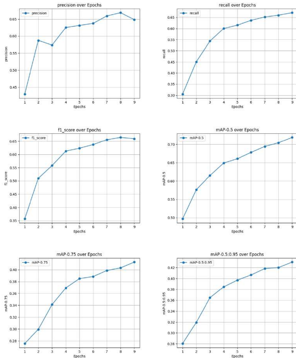
Figure 4.39: Plots per epoch for Faster R-CNN with MobileNetV3 (Thermal dataset)
