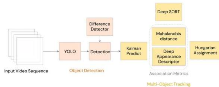
Figure 5.8: DeepSORT architecture [74]
