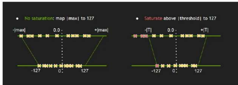
Figure 4.57: INT8 calibration [68]
