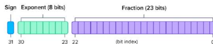
Figure 4.55: FP32 representation [69]
