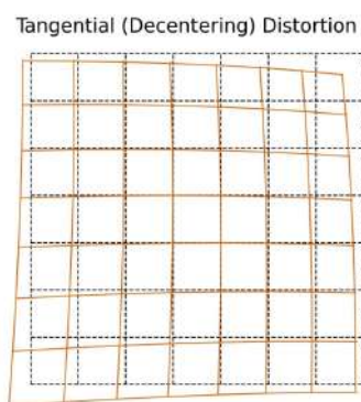
Figure 5.5: Tangential distortion [70]
