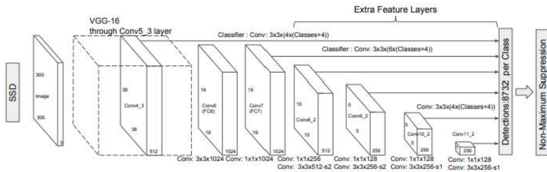
Figure 4.28: SSD architecture [63]
