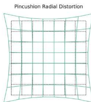
Figure 5.3: Positive (pincushion) distortion [70]
