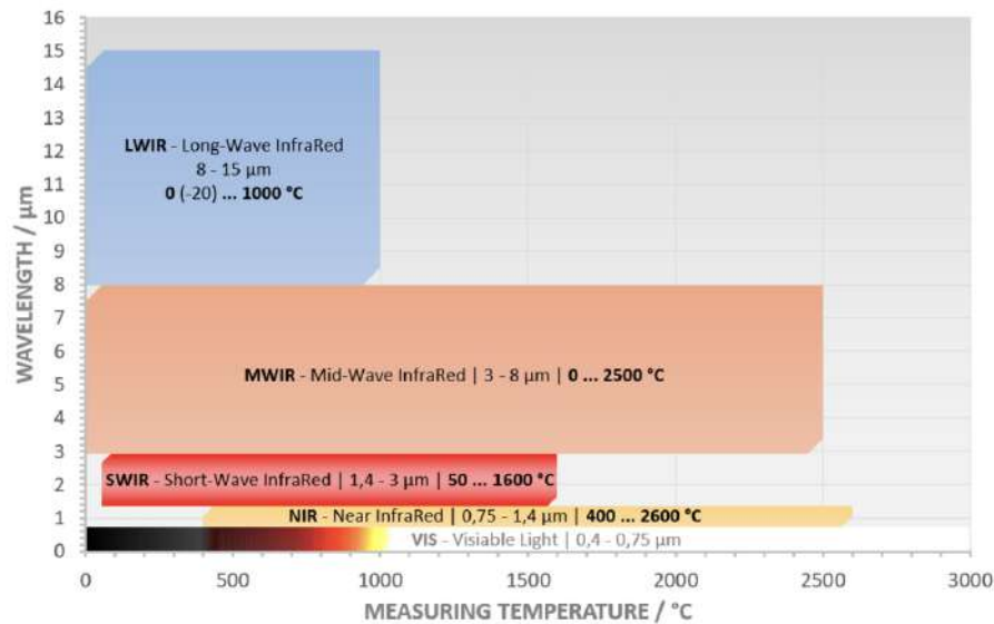
Figure 2.7: Infrared wavelength bands and their corresponding temperature ranges [16]
