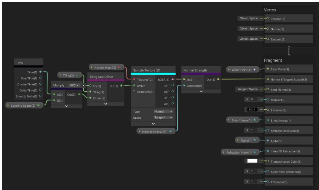
Figure 3.4.3: Water shadergraph.
