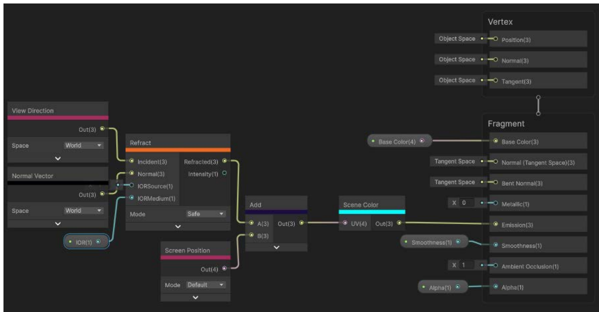
Figure 3.4.1: Glass shadergraph.
