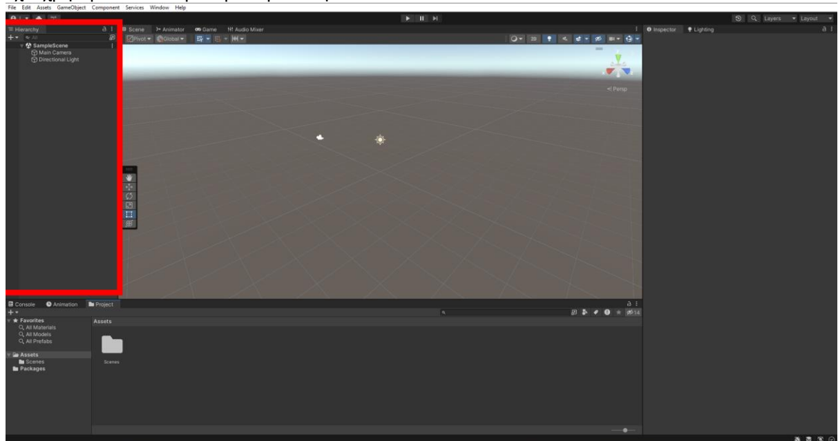
Unity Hierarchy
