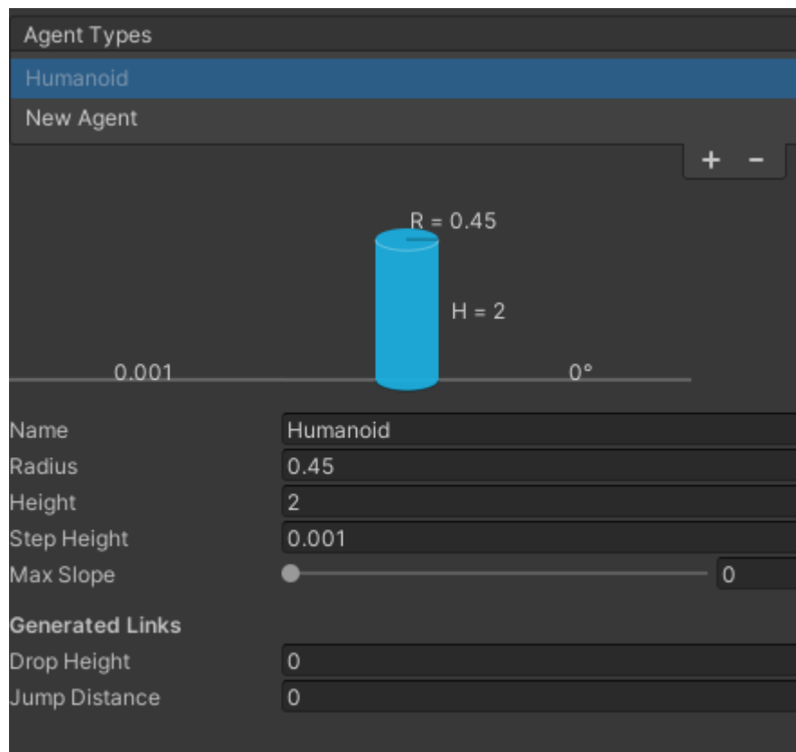
Agent Settings
