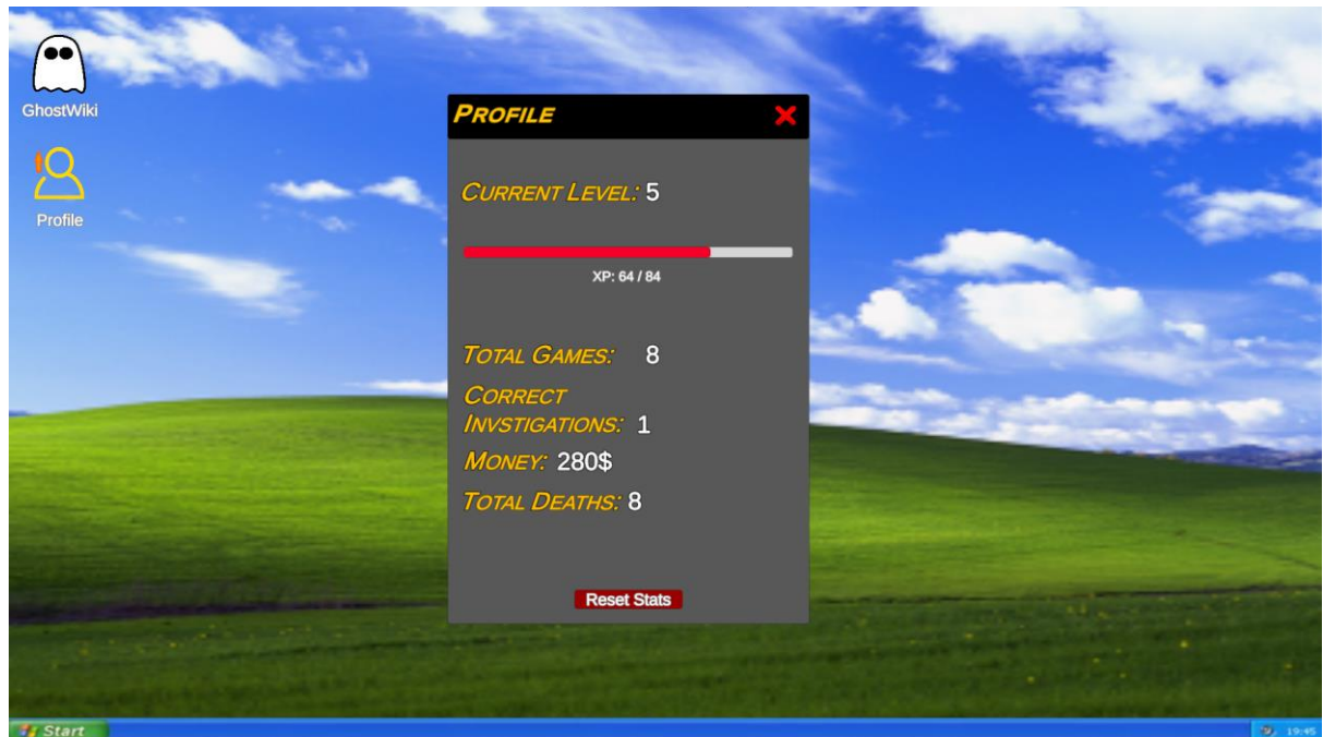
Profile App
