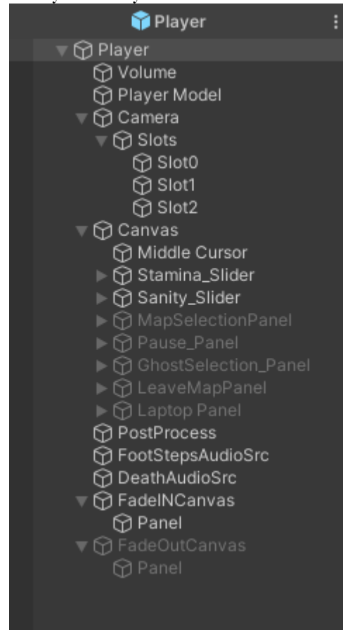
Player Prefab Hierarchy
