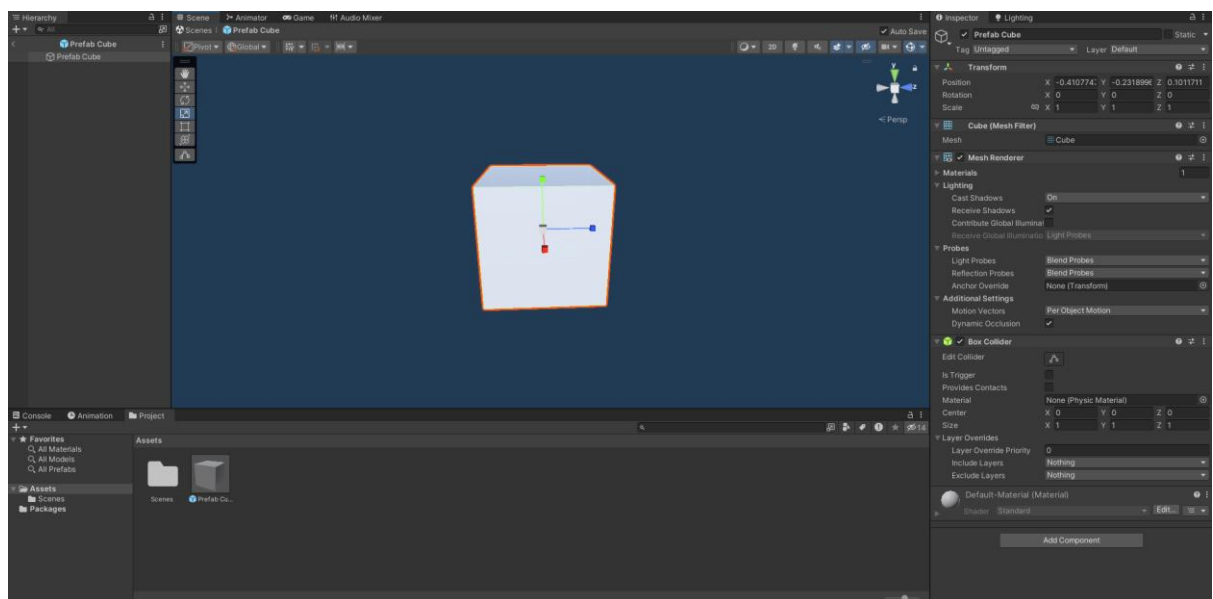
Onbject Prefab
