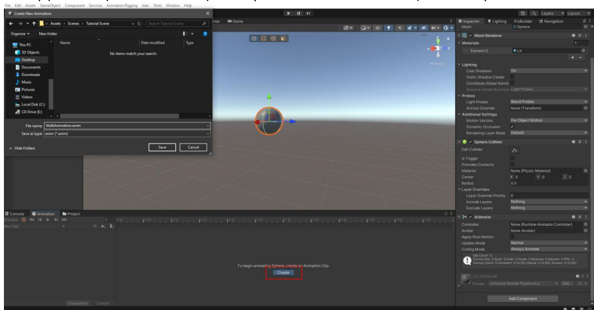
Create Animation
