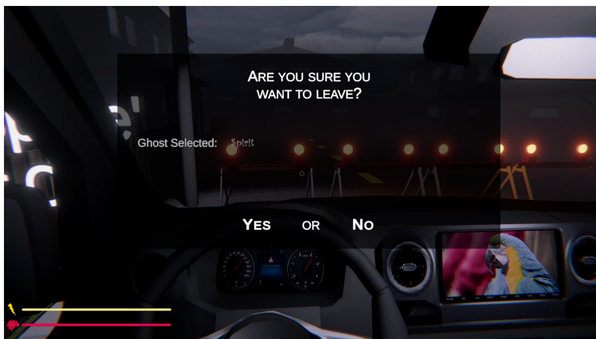
LeaveMapPanel
