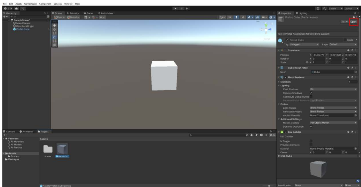
Prefab Inspector
