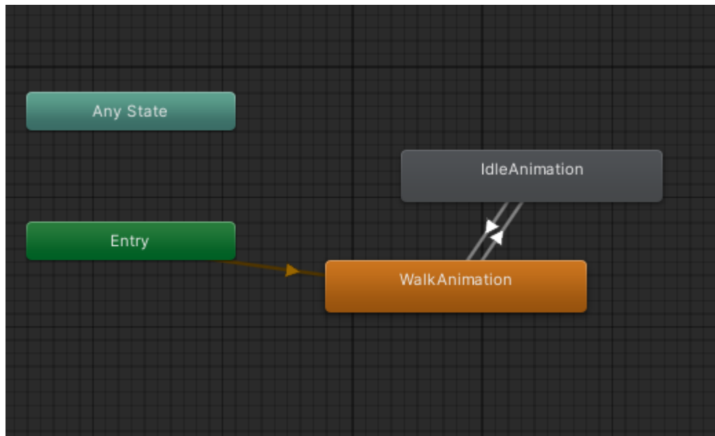
Animator Transition
