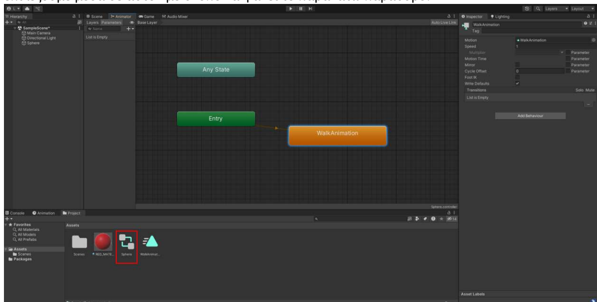
Animator Display
