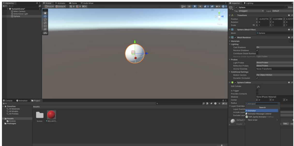
Animator Component
