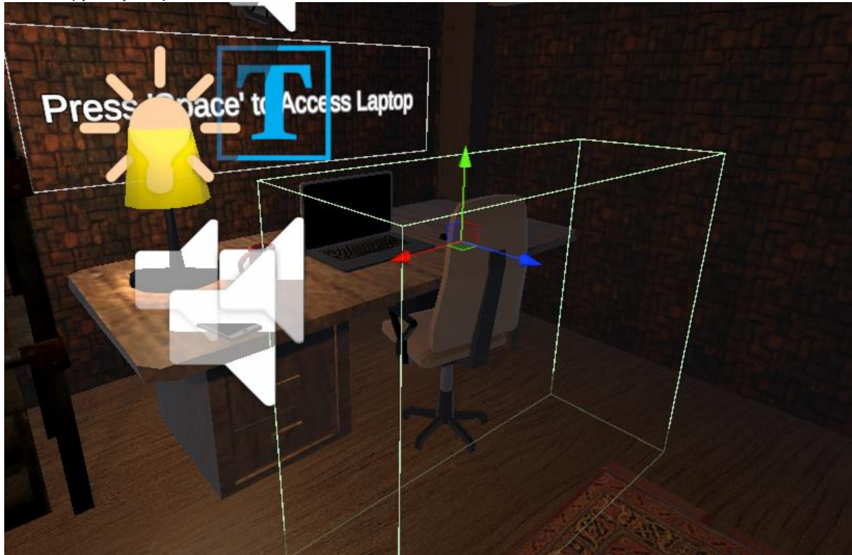
CameraSpot GameObject
