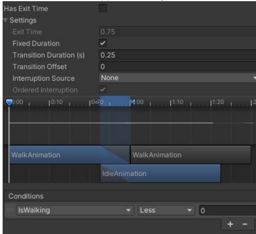
Animator Conditions
