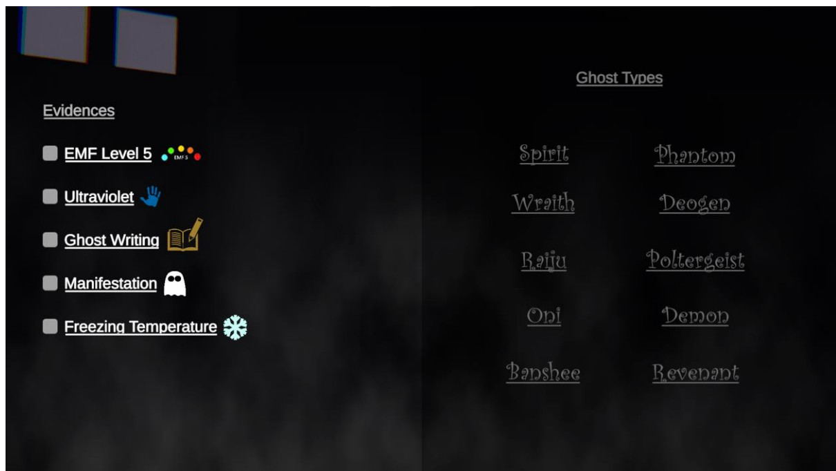
GhostSelectionPanel
