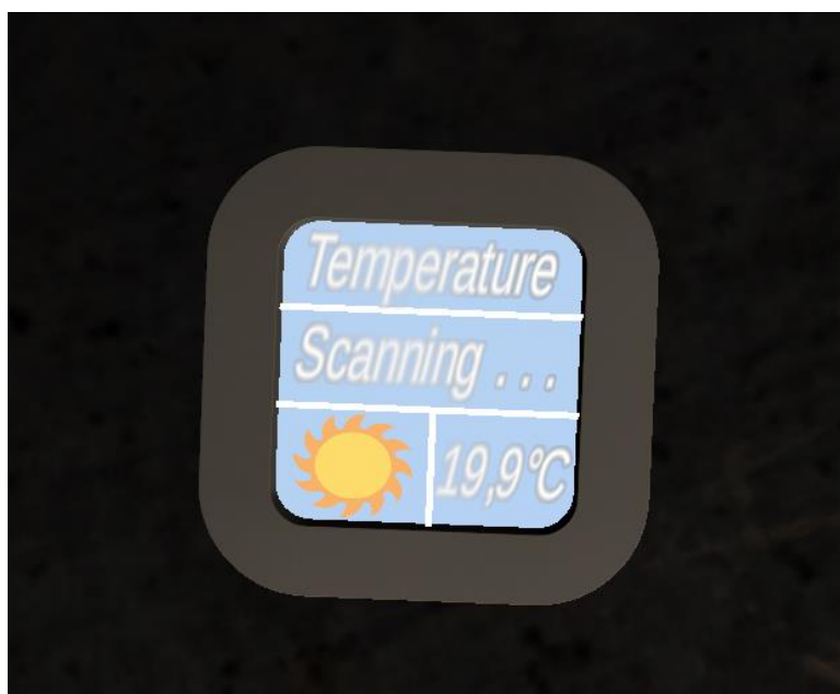
Thermometer Device
