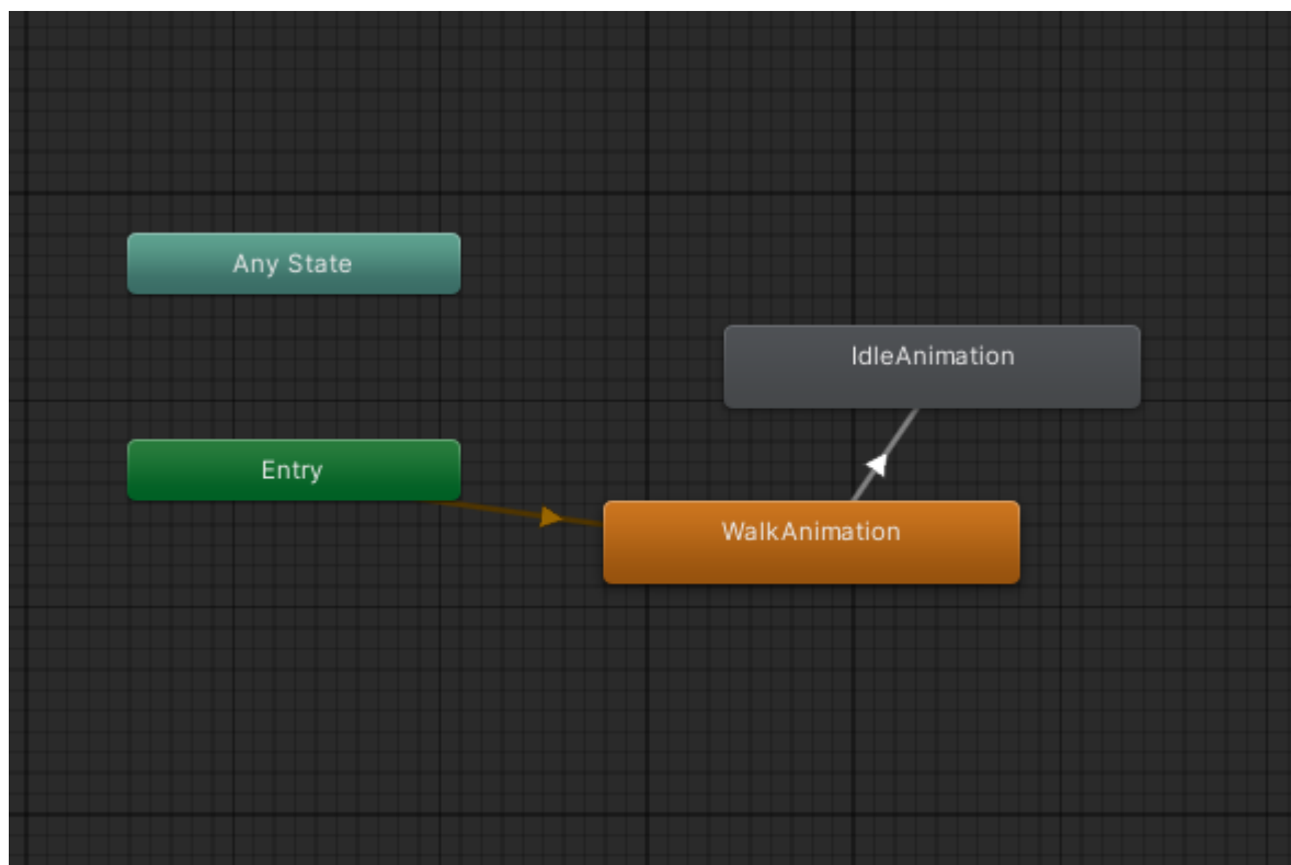
Animator
