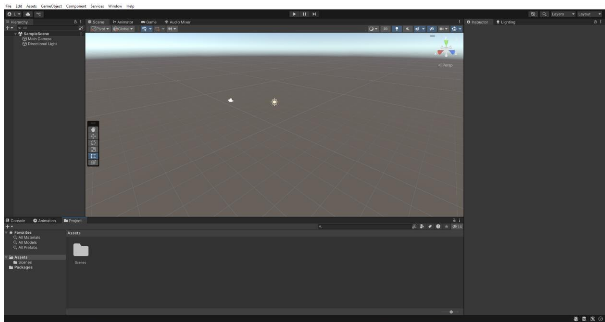
Unity Scene
