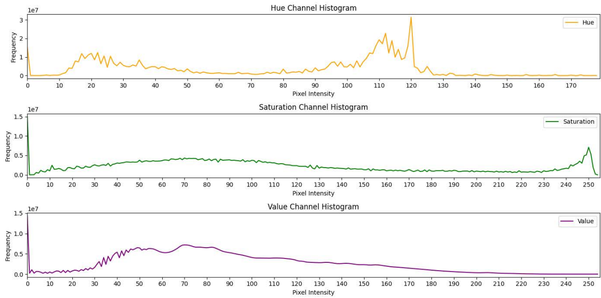
Figure 9: Histogram of Simple True Color HSV Channels
