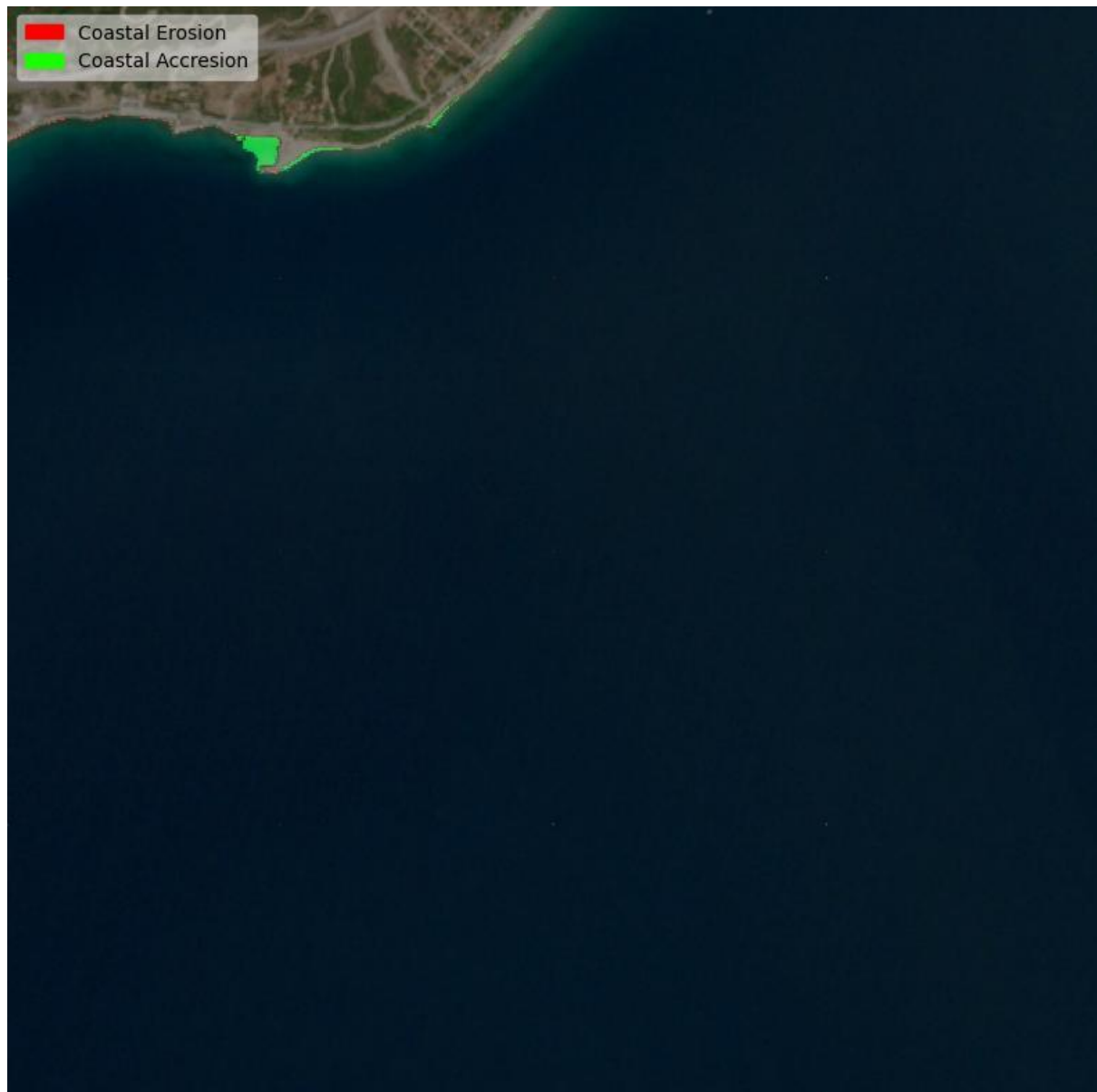
Figure 16: Coastal Fluctuations Visualization of Kiani Coast of Thessaloniki, Greece from 2017 to 2021
