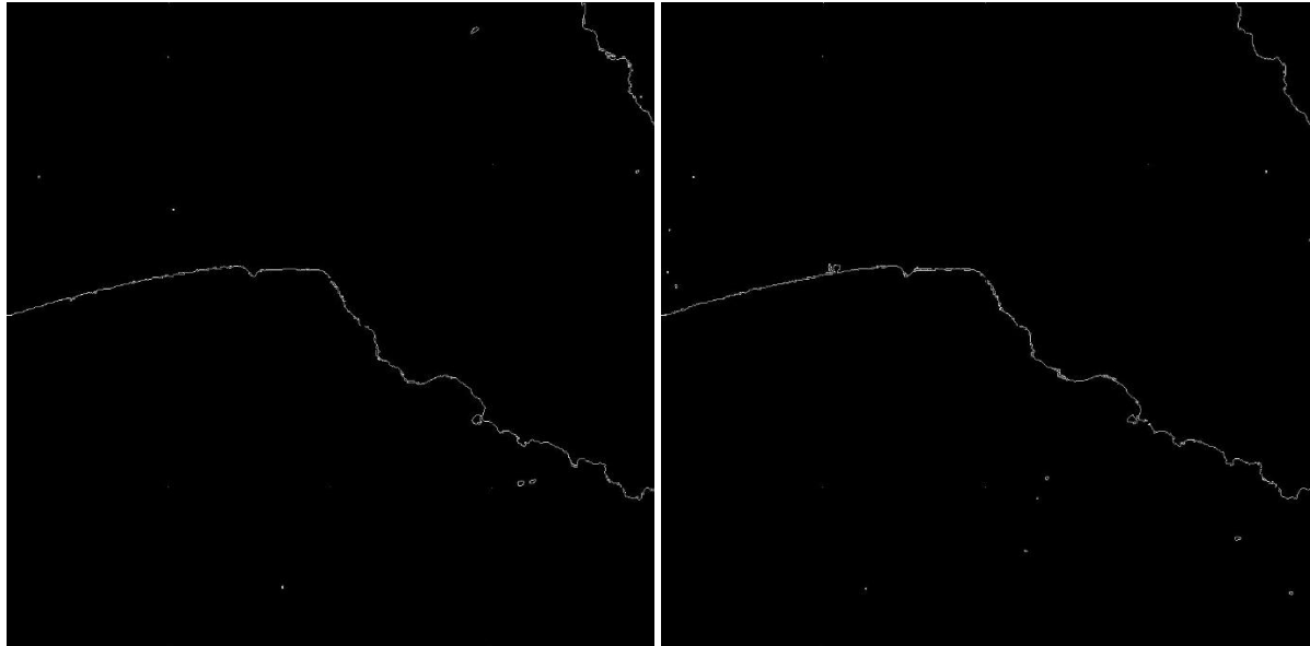
Figure 14: Detected Shorelines of Kalamaki Coast of Zakynthos, Greece in 2017 (left) and 2023 (right)
