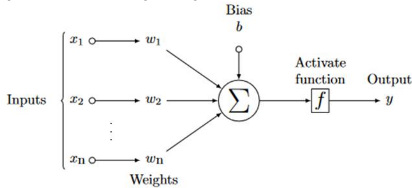
Figure 5: The internal workings of a single neuron in a neural network
