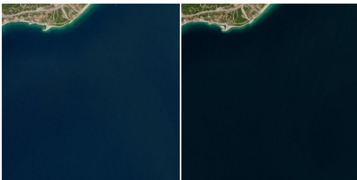
Figure 19: Satellite Images of Kiani Coast, Thessaloniki, Greece in 2017 (left) and 2021 (right)
