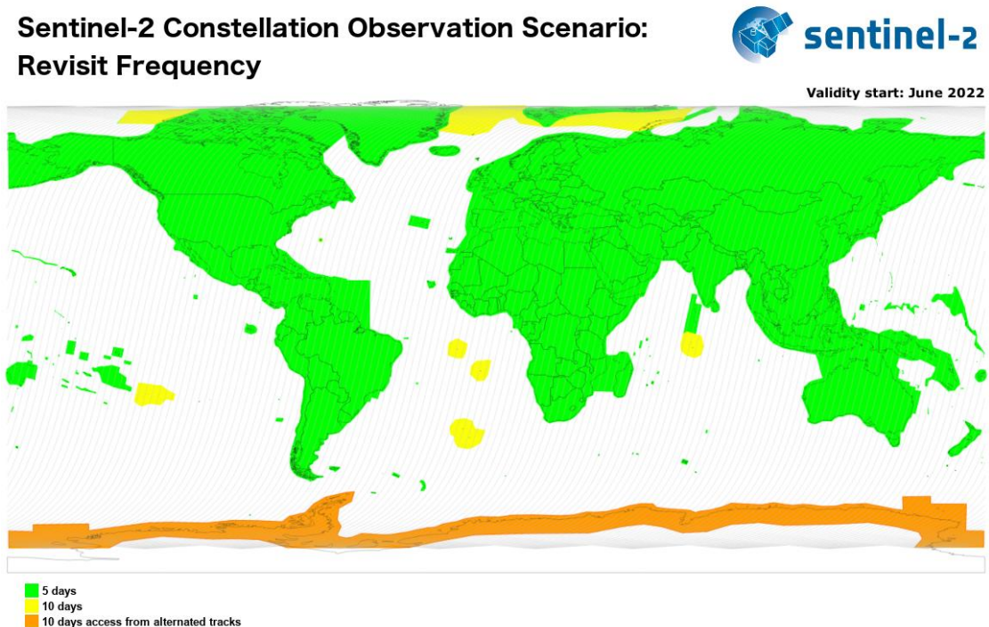
Figure 2: The coverage and revisit time foreseen for Sentinel-2 MSI acquisitions. [Credits: ESA]
