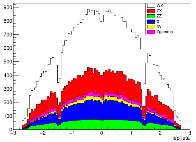
Stacked Histograms
