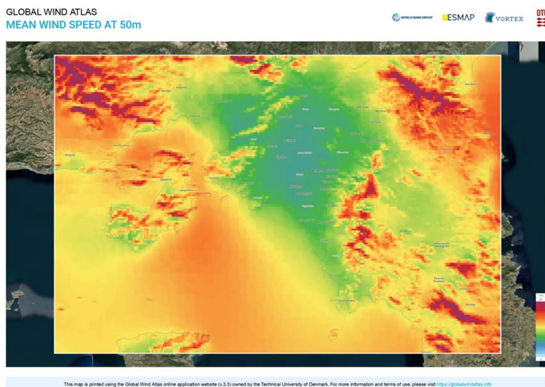
Figure 5.2: Mean wind speed in Attiki
