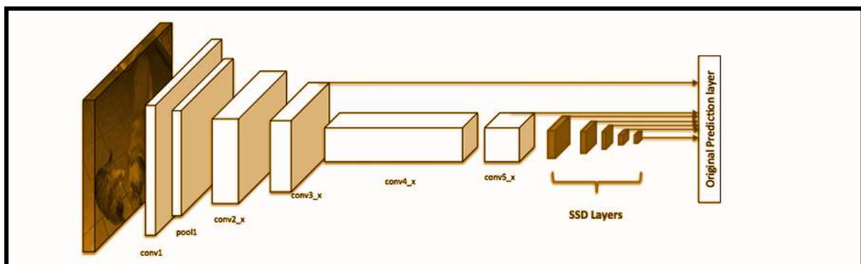
Fig. 2.2.3 Single Shot detector structure.
