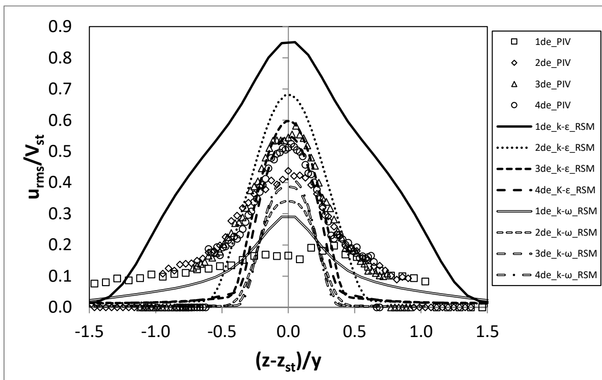
Figure 5-33: Normalized u_{rms} , Re=7700 , L/d_e=7.5
