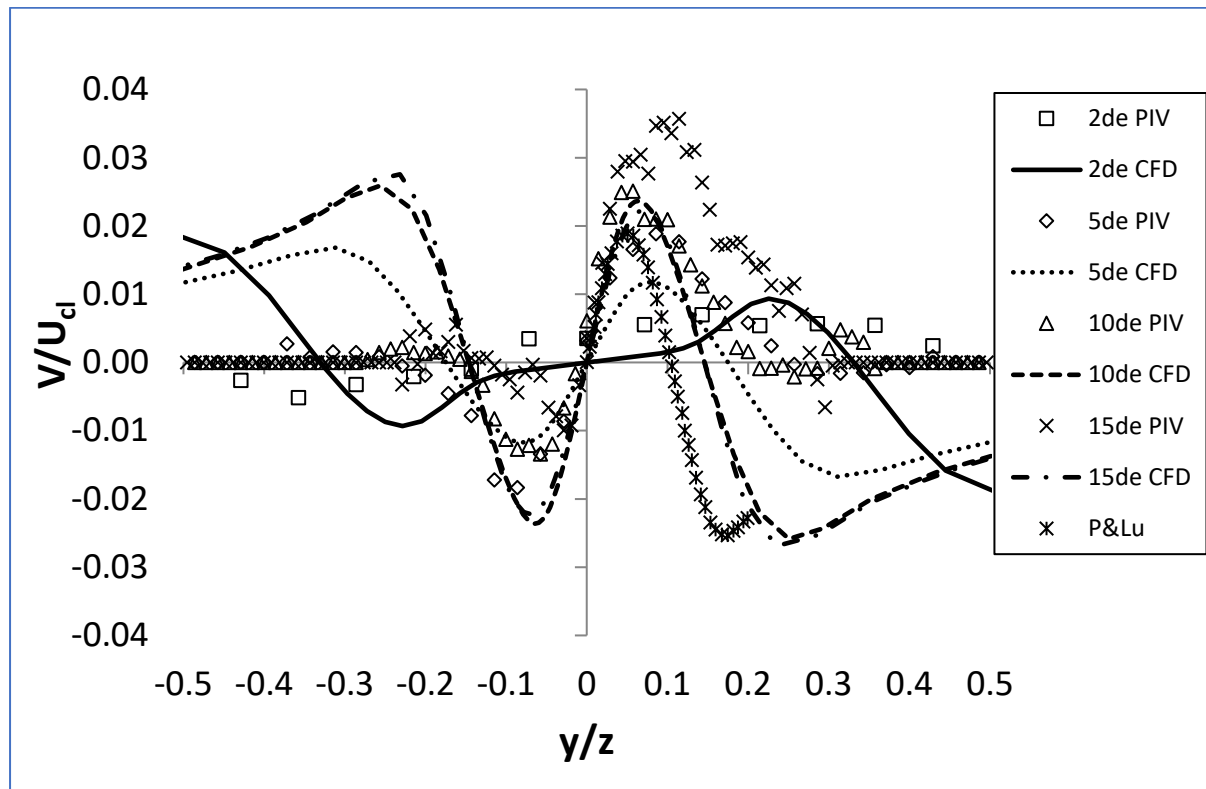
Figure 4-15: Normalized cross stream profiles of mean velocity V , Re\ 3300
