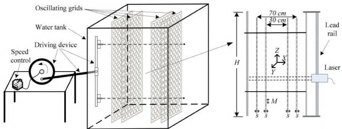
Figure 2-3 Sketch of the experimental system employed by Li et. al. [23] for the production of homogeneous and isotropic turbulence using symmetrically placed oscillating grids in a water tank.
