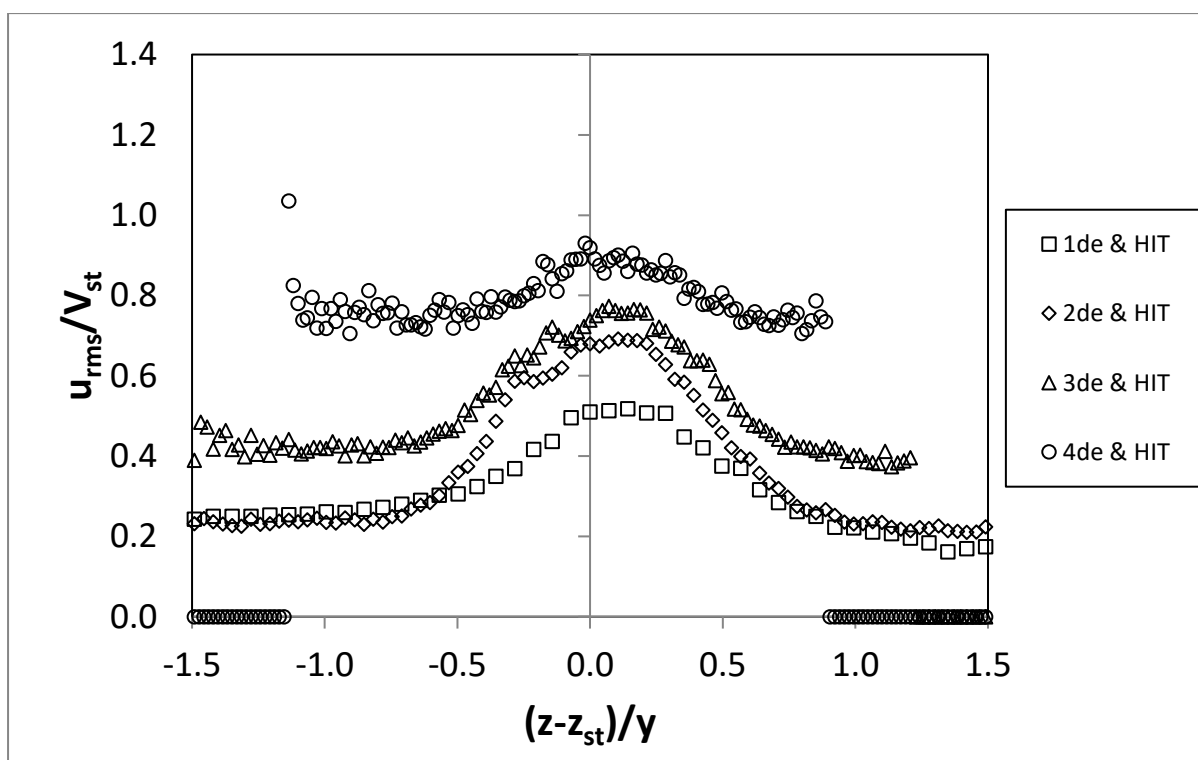
Figure 5-63: Normalized u_{rms} , Re=5500 under HIT , L/d_e=7.5
