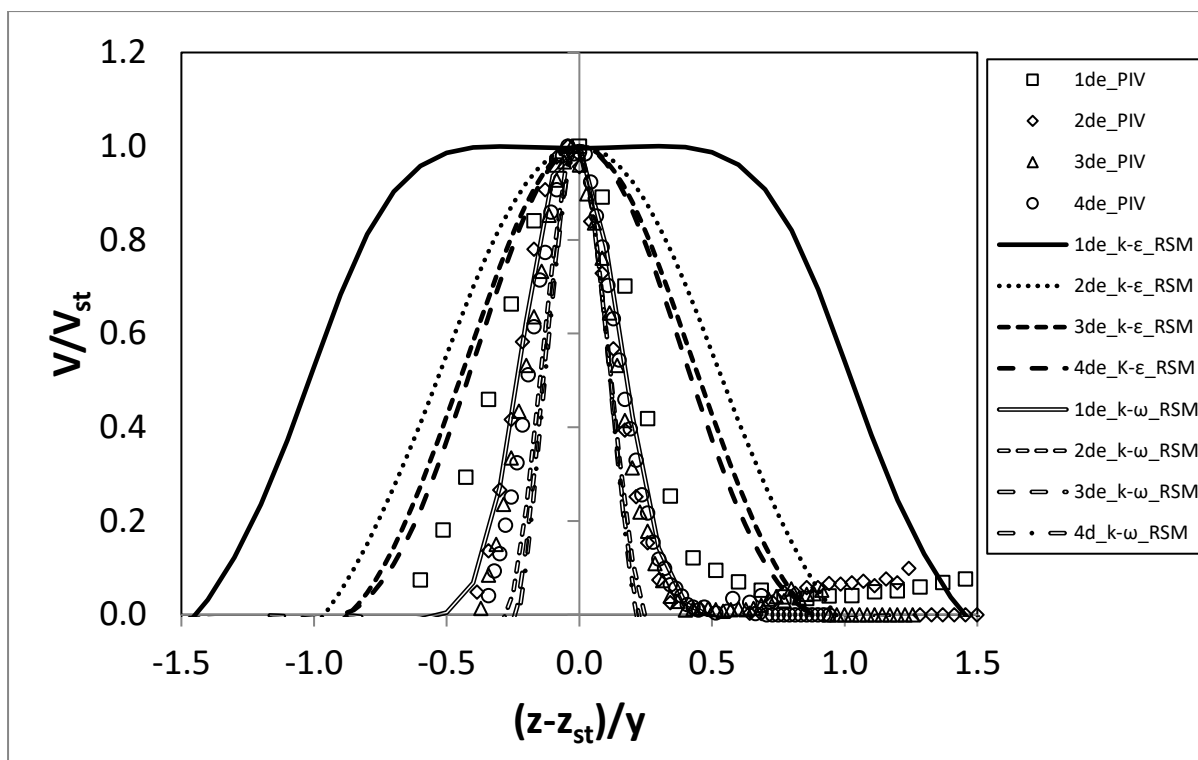
Figure 5-22: Normalized mean radial velocity V , Re=5500 , L/d_e=5
