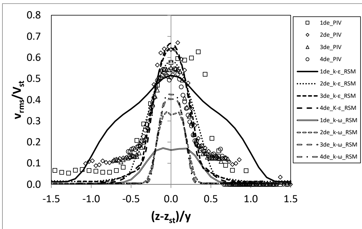
Figure 5-27: Normalized v_{rms} , Re=7700 , L/d_e=5
