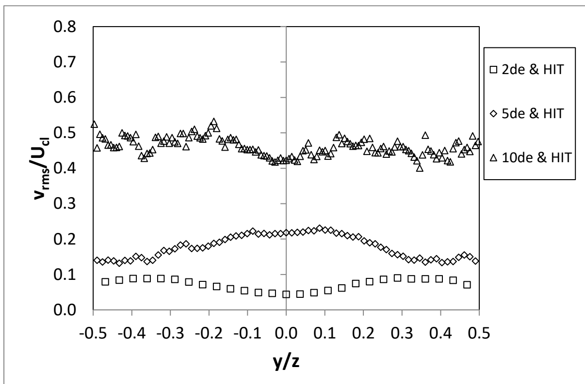
Figure 4-34: Normalized cross stream profiles of v_{rms} , Re 3300 under HIT
