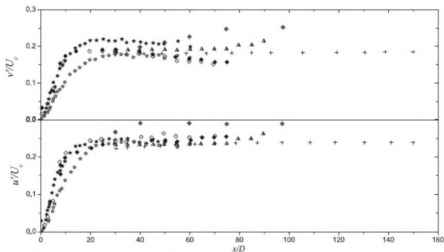
Figure 2-14 Turbulent intensities/normalized stresses axial evolution, aggregate of experimental data adapted by Ball et. al [75]
