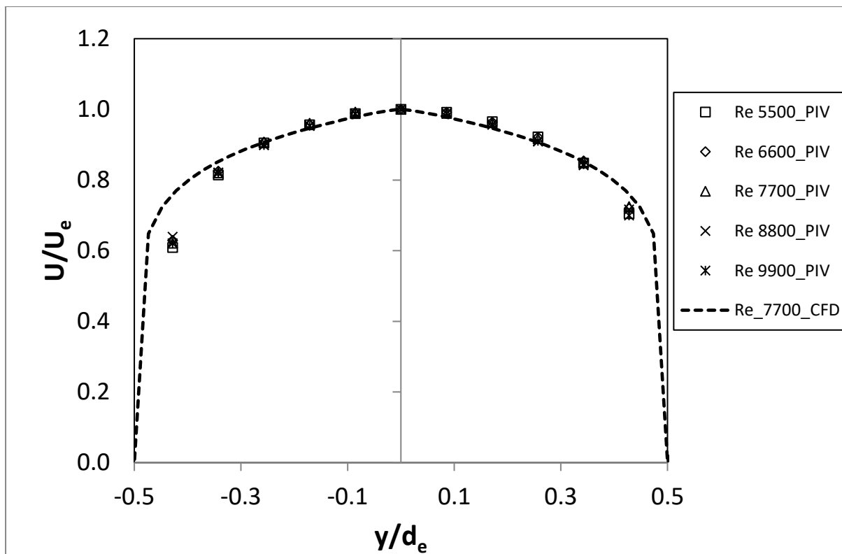
Figure 5-3: U_e velocity profile at the pipe exit, L/d_e=5 , PIV & CFD Data
