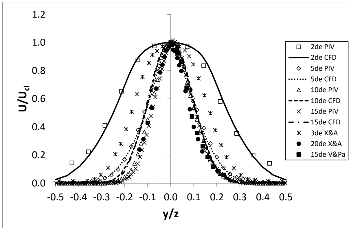
Figure 4-13: Normalized cross stream profiles of mean velocity U , Re = 3300
