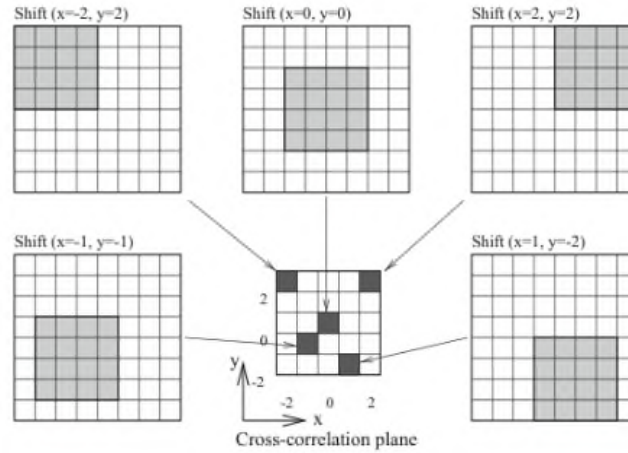
Figure 3-9: Tracing of a 4px \times 4px interrogation area within an 8px \times 8px search area to produce a 5px \times 5px correlation map. The central matrix is the correlation map. (Image source [131])
