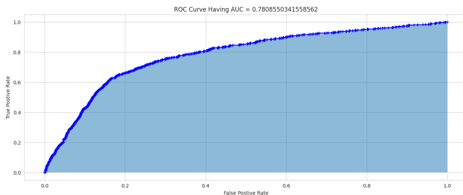
Figure 4.4: LightGBM Classifier ROC Curve
