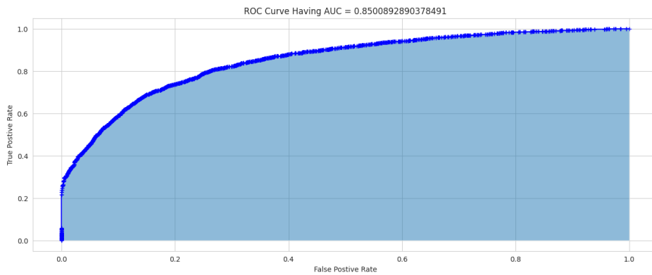
Figure 4.11: CNN-LSTM Classifier ROC Curve.
