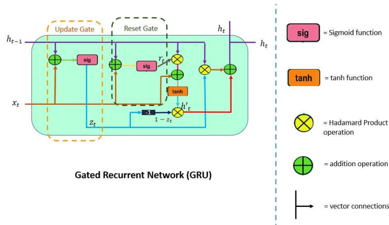
Figure 3.7: GRU classifier
