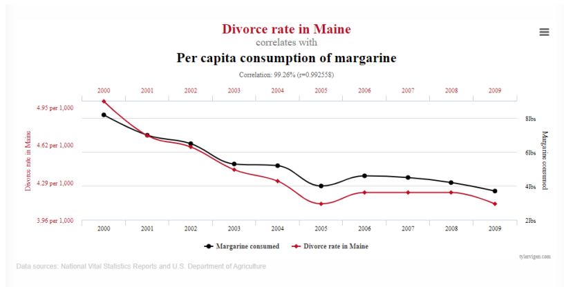
Figure 2.1: Spurious Correlations [2]
