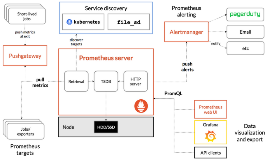
Figure 5.6: Prometheus echosystem components
