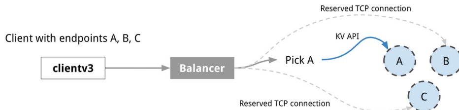
Figure 3.3: gRPCv1.0 Balancer
