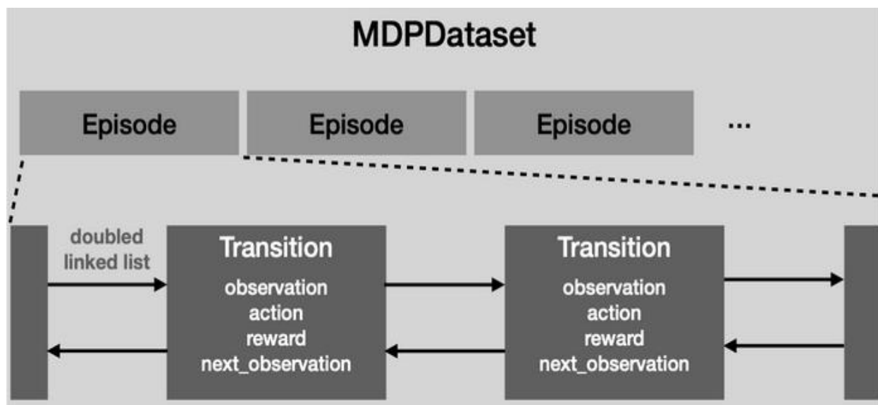
Figure 9: MDPDataset structure [16]
