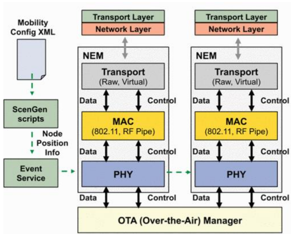
Figure 7: EMANE architecture [14]
