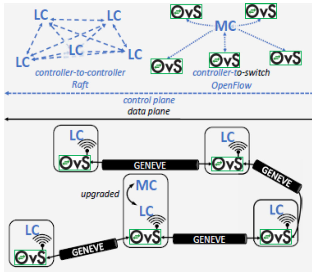
Figure 1: SDN-MANET architecture [1].
