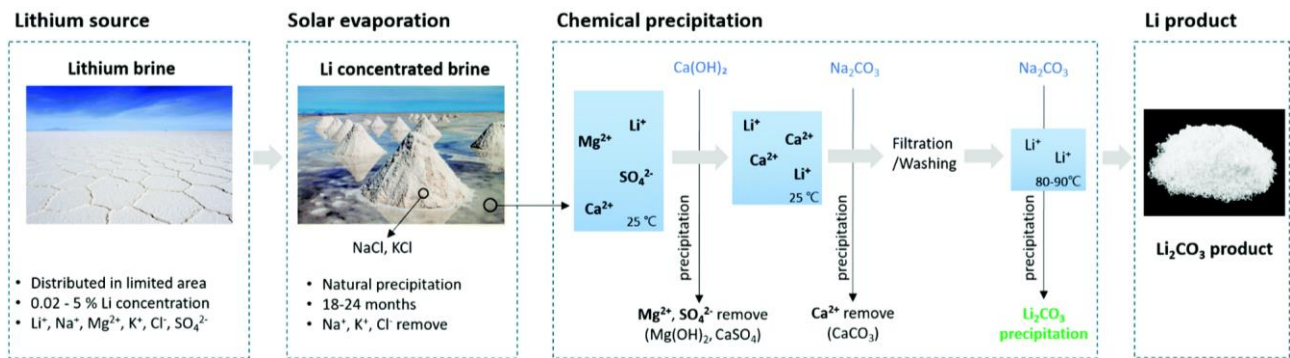
Figure 23: Lithium extraction via chemical precipitation [129].
