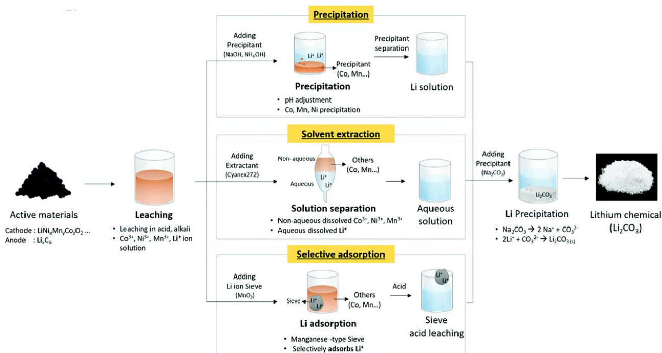
Figure 29: Lithium recycling from pretreated Li-ion battery components, using hydrometallurgy [129].
