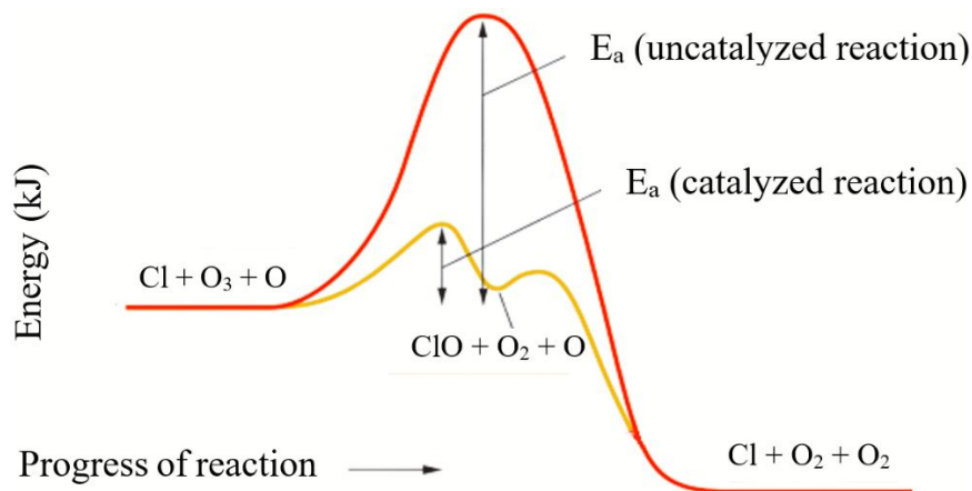
Figure 5: Depiction of the impact on the activation energy of the ozone breakdown reaction, due to catalytic activity [10], [104].
