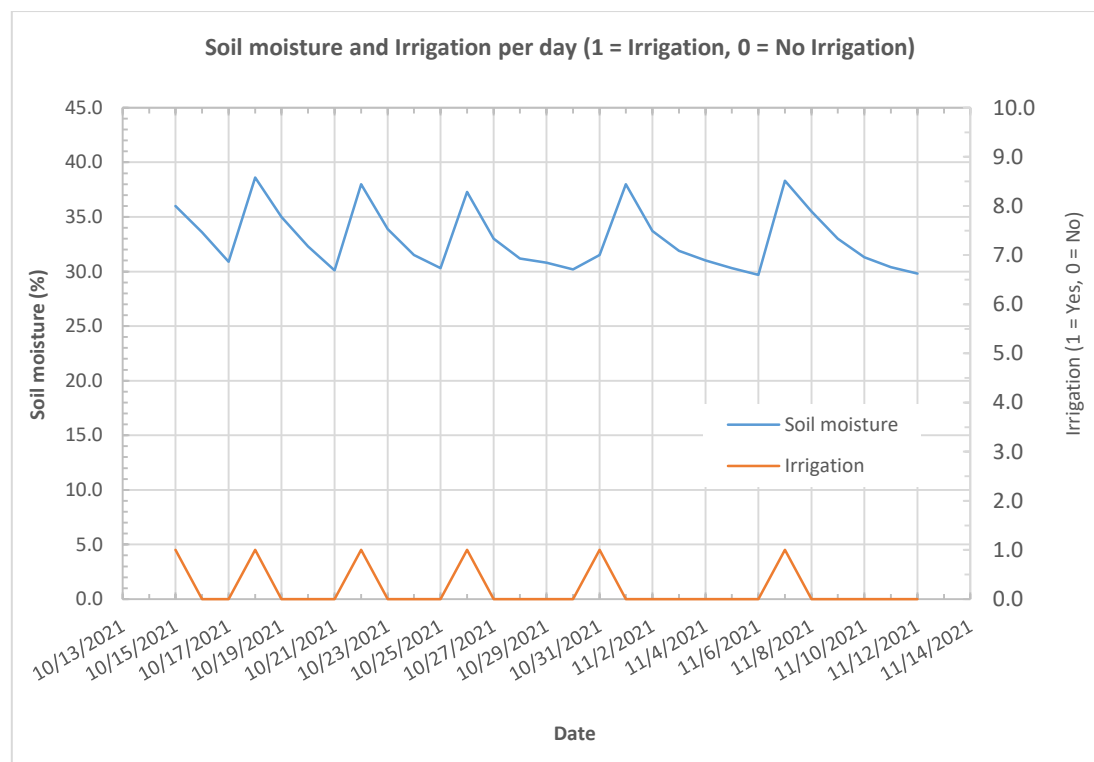
Figure 150: Automated irrigation using FMMIS
