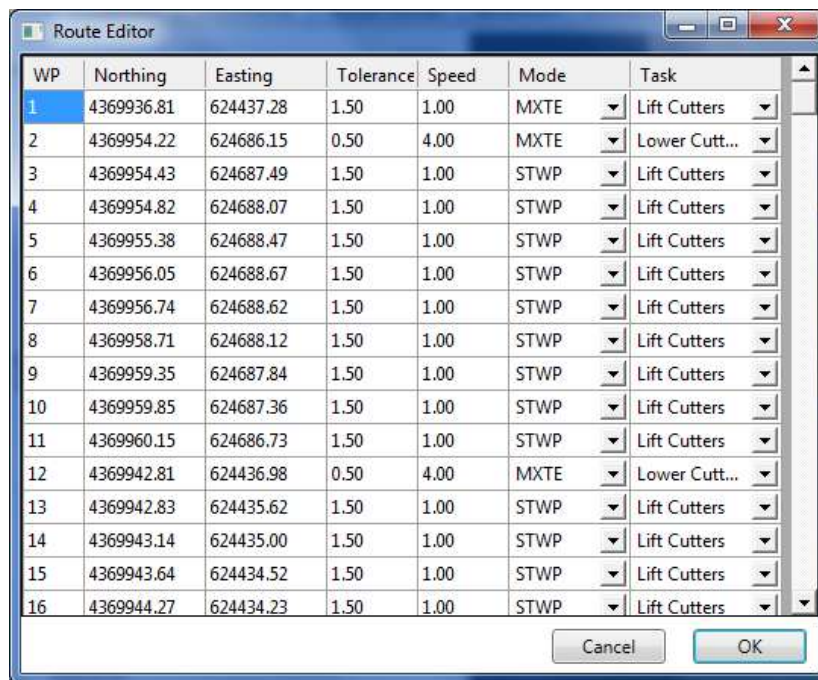
Figure 106: Route editor dialog
