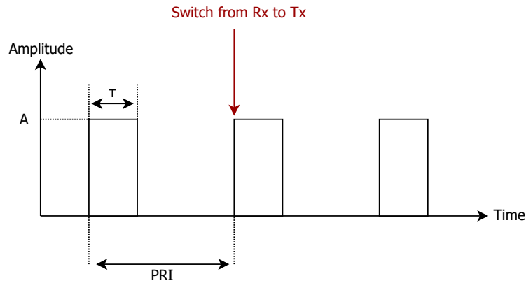
Figure 3.6: Baseband rectangular pulses of width \tau and amplitude A , each transmitted every PRI seconds. After the end of the first PRI interval, the antenna is switching to transmitting mode.
