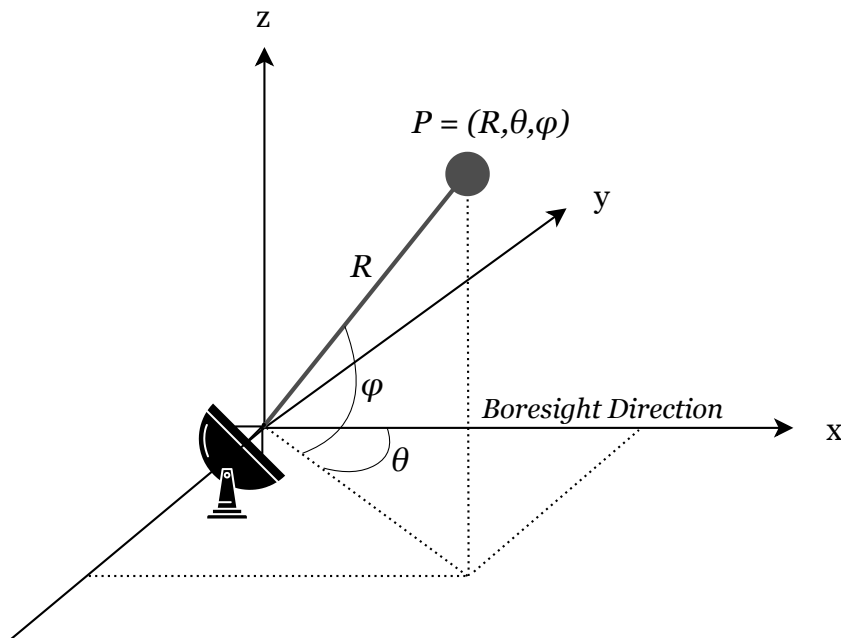
Figure 3.3: The spherical coordinate system used for radar measurements, with the target located at point P [12].
