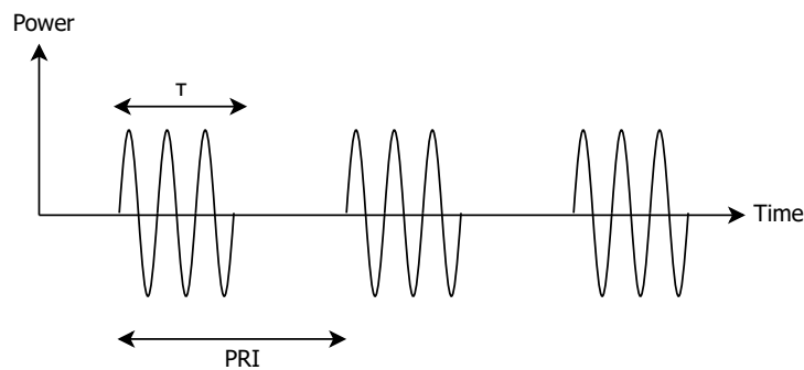
Figure 3.5: Transmission of passband modulated pulsed waveforms. Each pulse is of width \tau and is repeatedly emitted after an interval of PRI seconds.
