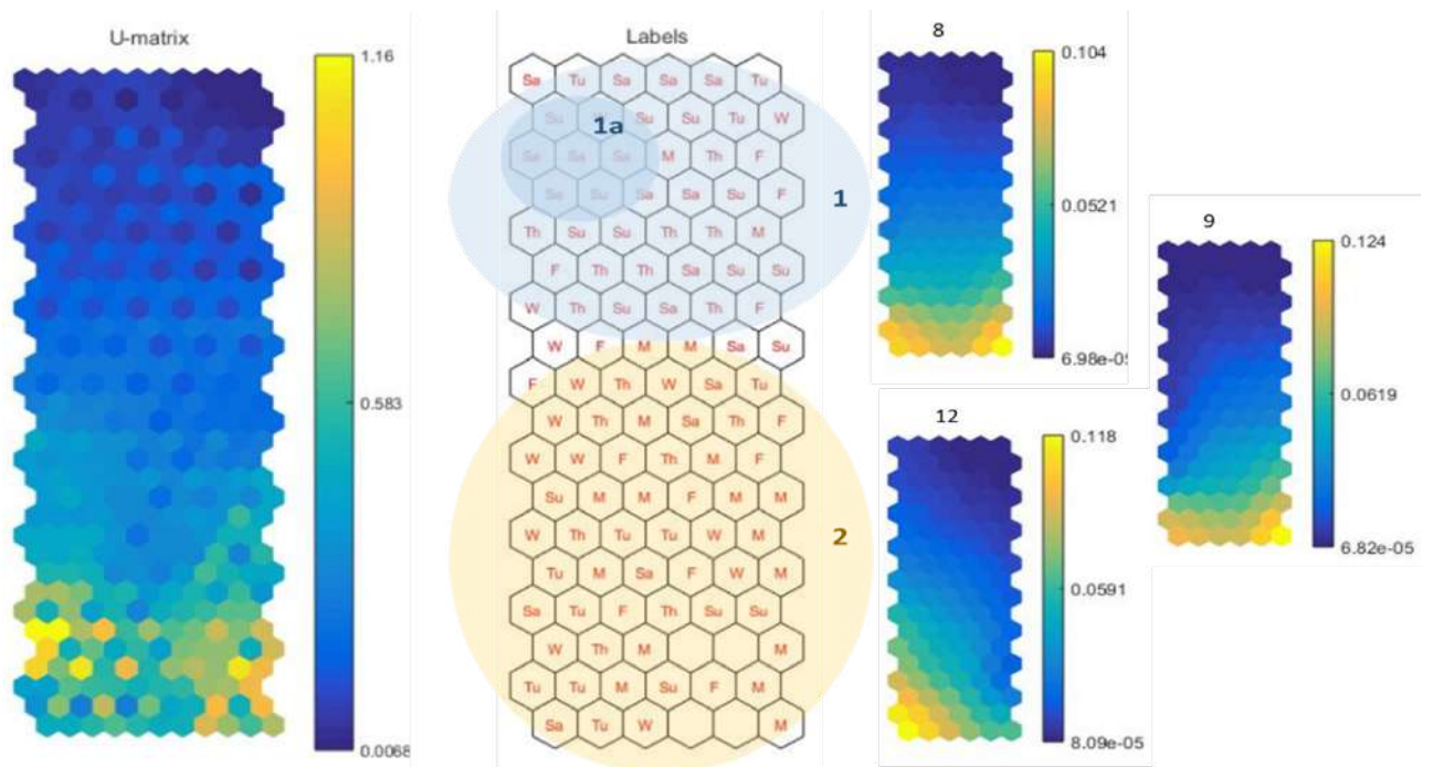
Figure 2.5. It is depicted the SOM map results: U-matrix, Labels, feature 8 consumption at offices working hours, feature 9 consumption at banks working hours, and feature 12 consumption at shops working hours (Approach 3).
