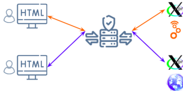
Figure 2.6: Reverse Proxy Server traffic forwarding to different servers and clients
