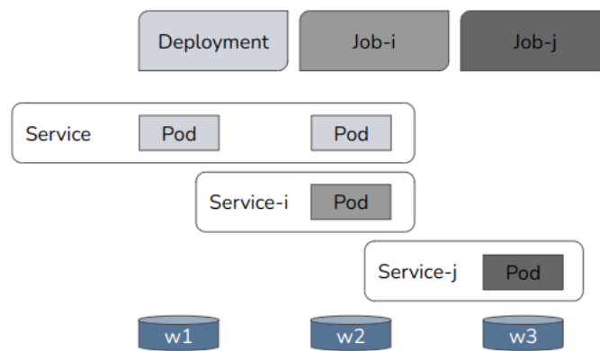
Figure 2.2: Kubernetes Deployment and Jobs Workload resources
