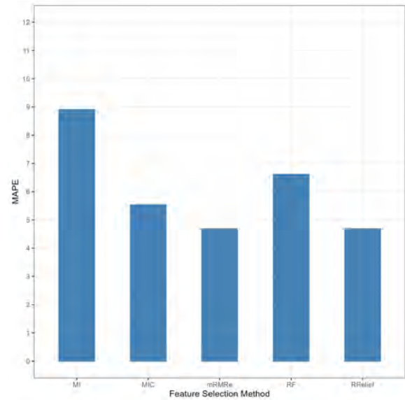
(b) MAPE of the top 40 features.
