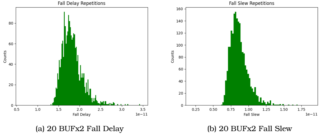
Figure 5.4: 20 BUFx2 Fall Results
