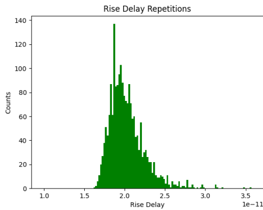
(a) 4 BUFx24 Rise Delay
