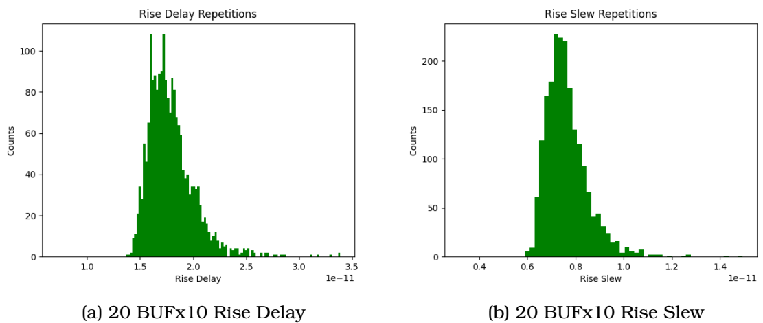
Figure 5.7: 20 BUFx10 Rise Results
