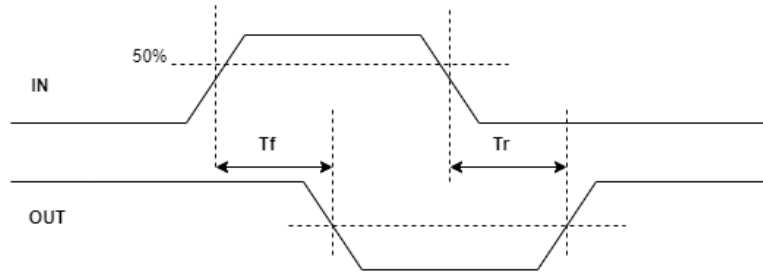
Figure 2.10: Rise and Fall Propagation Delay
