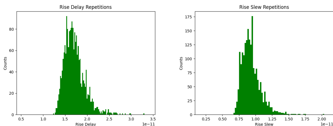
(a) 20 BUFx2 Rise Delay
