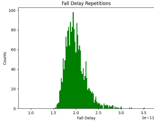
(a) 20 BUFx10 Fall Delay
