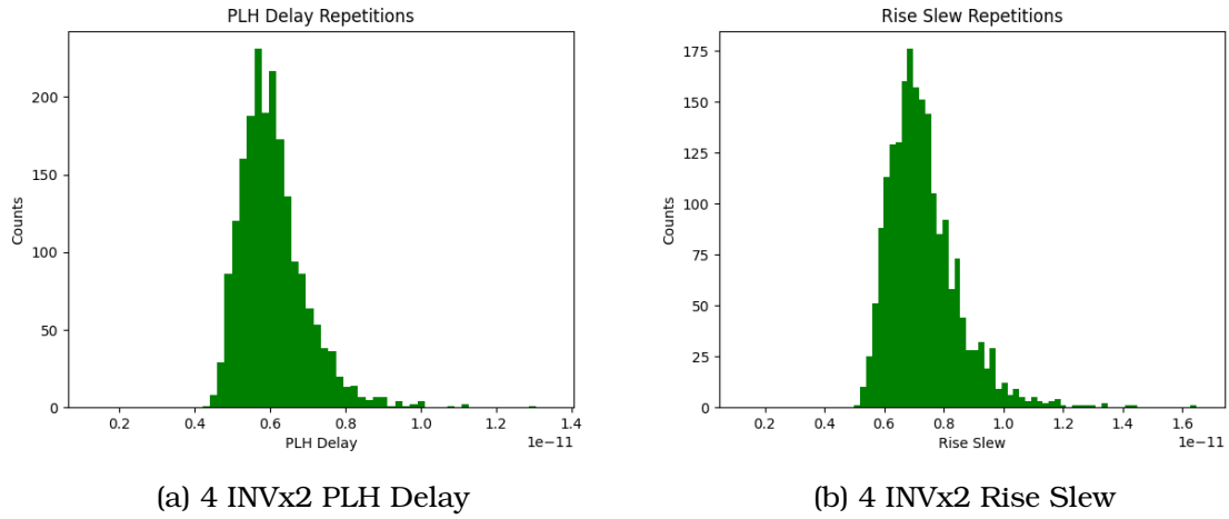
Figure 5.13: 4 INVx2 Rise Results
