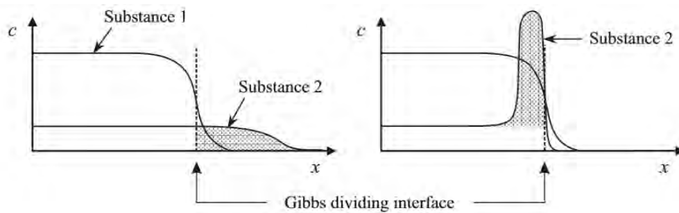
Figure 3.6: Concentration profiles for two substances with respect to the dividing plane, adapted from [120].
