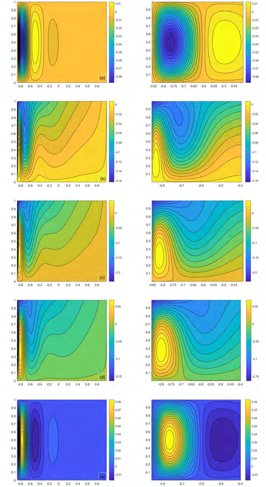
Figure 6.10: Iso-contours of tangential velocity, \Re[u_{\theta 1}(\delta/H, x, t) e^{i2\pi t}] , for t = 0 (a), t = 0.125 (b), t = 0.25 (c), t = 0.375 (d) and t = 0.5 (e). The x -axis is x = -\cos(\theta) and the y -axis \delta/H . Figures on the right are magnifications of those on the left close to the rim.
