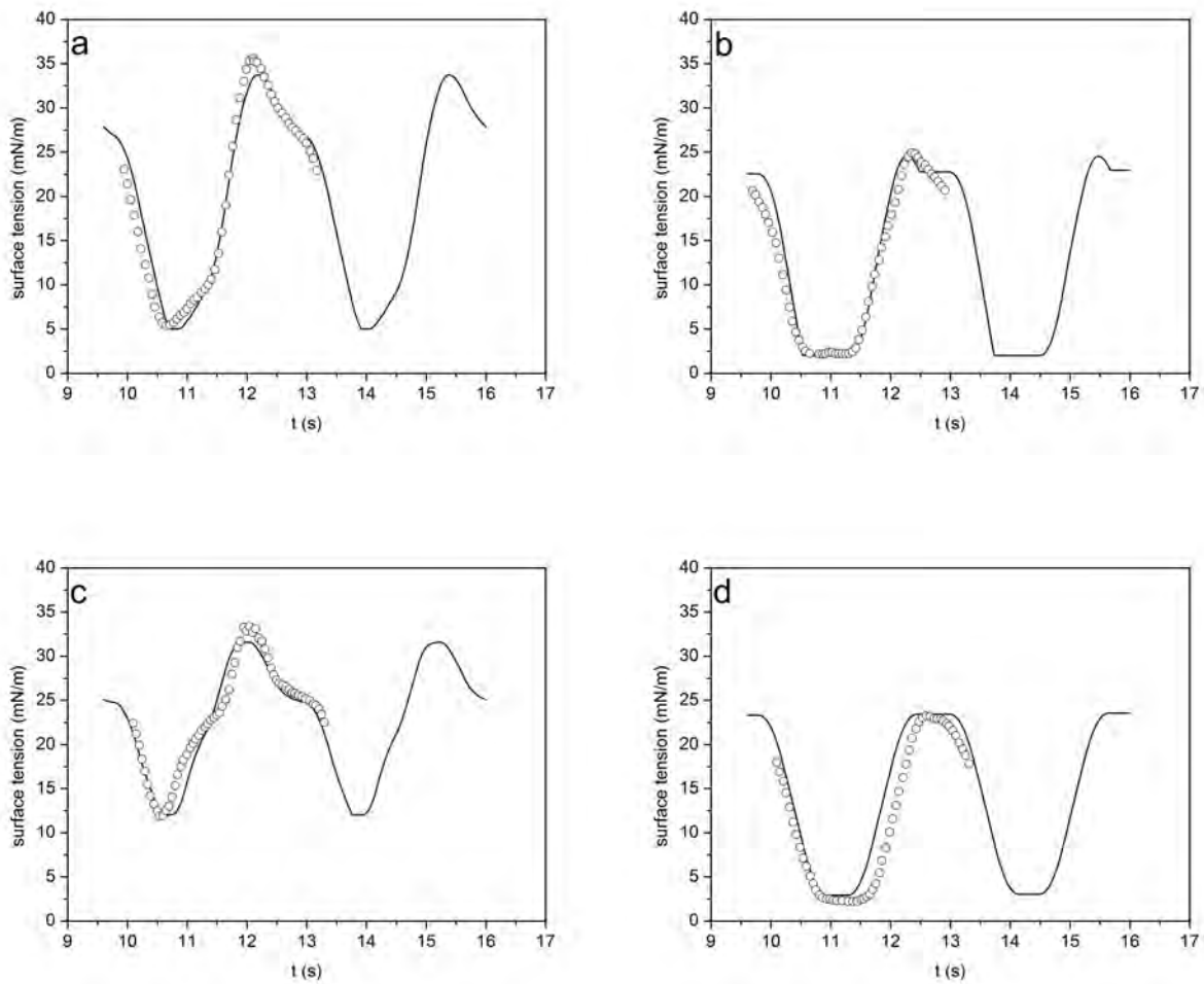
Figure 5.4: Predictions of surface tension variation with time during two consecutive cycles (solid lines), compared to the experimental data (circles) from ref. [149] : a) C = 0.5 \text{ mg ml}^{-1} (humid air), b) C = 0.5 \text{ mg ml}^{-1} (dry air), c) C = 2 \text{ mg ml}^{-1} (humid air), d) C = 2 \text{ mg ml}^{-1} (dry air).
