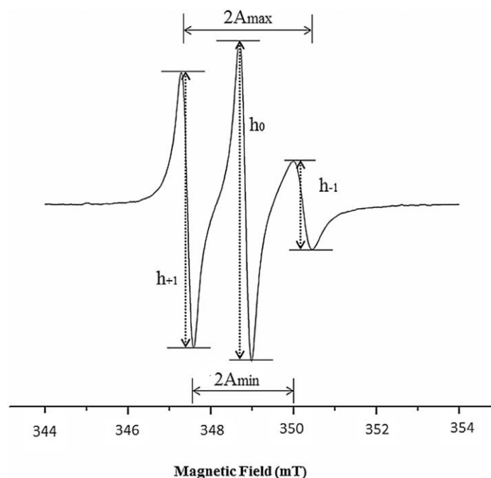
Figure 29. Illustration of a typical EPR spectrum of a nitroxide spin-probe with the three distinct peaks. Parameters A_{max} and A_{min} are also presented [415].
