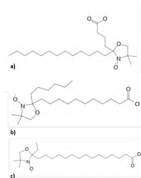
Figure 28. Molecular structures of the three nitroxides that were used as free radical in the present study namely, a) 5-DXA, b) 12-DXA and c) 16-DXA (source: https://spectrabase.com/ ).
