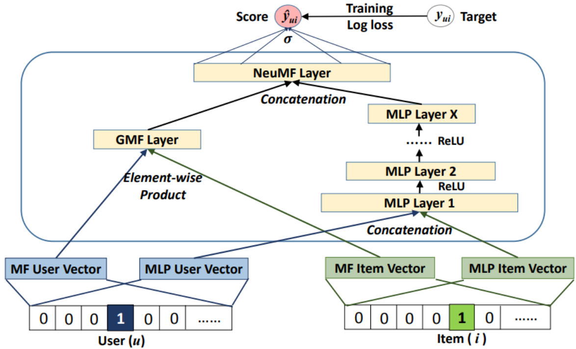
Figure 5.3: Neural matrix factorization model.[11]
