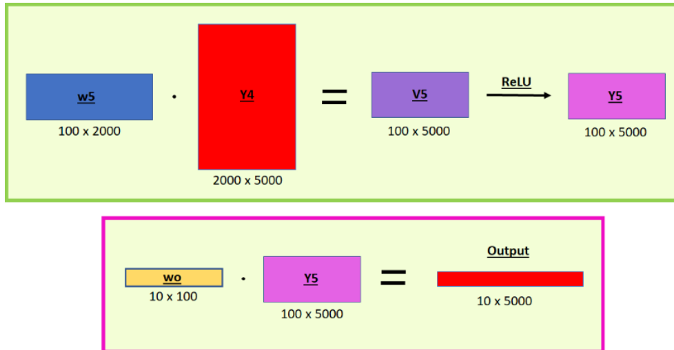
Figure 21b: Y4 is multiplied with W5 and passed through the ReLU function, whose result is then multiplied with W0 ; their product is a matrix that contains each image's probability of recognizing classes 0-9.
