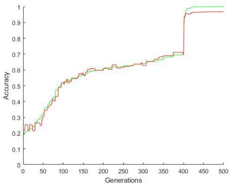
Figure 16a: Accuracy of our GA-CNN with 5000 training images. After 400 generations we performed BP to our model to upgrade the accuracy
