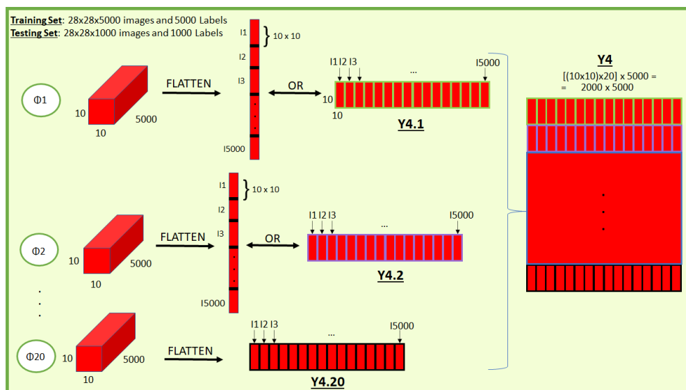
Figure 21a: here there are 5000, 28x28 training images (I1-I5000) that are convoluted with each filter of the convolutional layer ( \Phi 1 - \Phi 20 ); each result is passed through ReLU and mean-pool functions and then, it is flattened into a short and fat matrix (Y4.1-Y4.20). These matrices are put together to form Y4.
