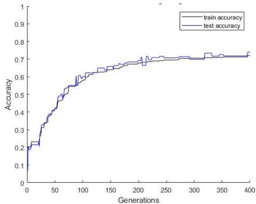
Figure 16d: Accuracy of our GA-CNN with 2500 training images
