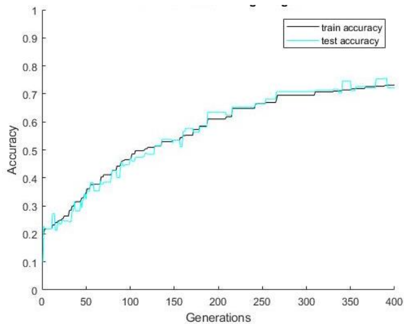
Figure 16c1: Accuracy of our GA-CNN with 1000 training images
