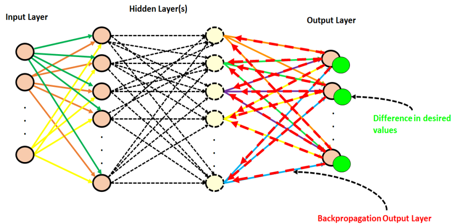
Figure 3: Training of CNN with backpropagation
