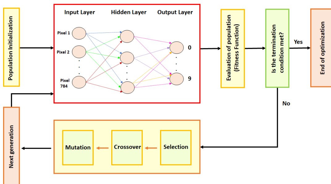
Figure 12: Genetic CNN
