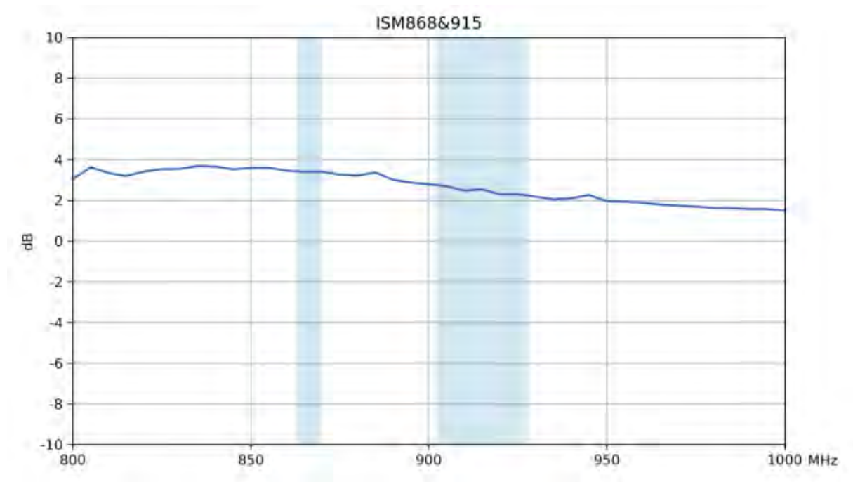
Figure 2.8: Peak gain.
