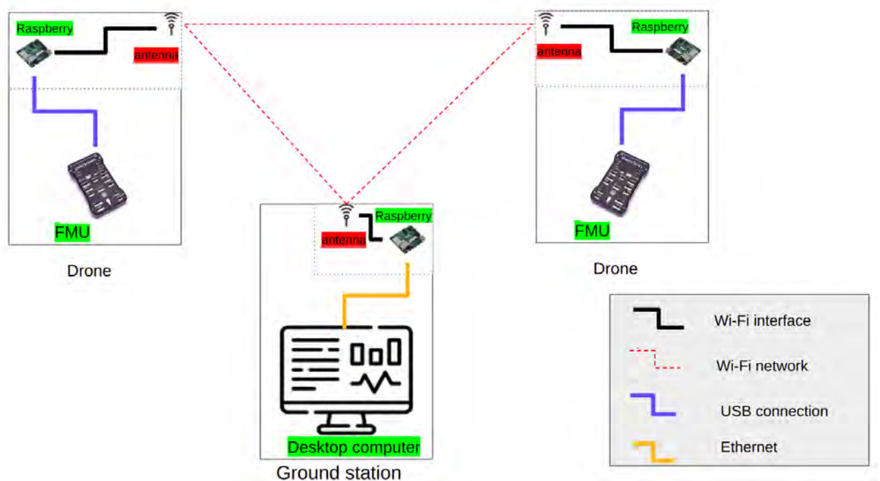
Figure 3.1: System architecture
