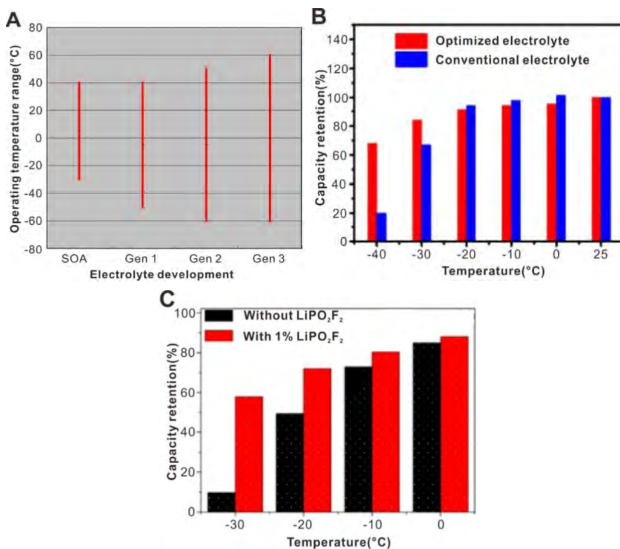
Figure 4.2. A) Different generations of electrolytes [298], B) Capacity retention of optimized and conventional electrolytes [308], C) Importance of using \text{LiPO}_2\text{F}_2 as additive in electrolyte [307].
