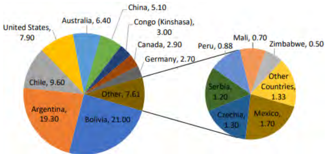
Figure 6.3. Lithium resources [563].
