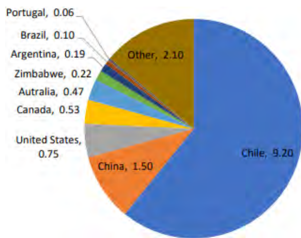
Figure 6.2 Lithium reserves [563].
