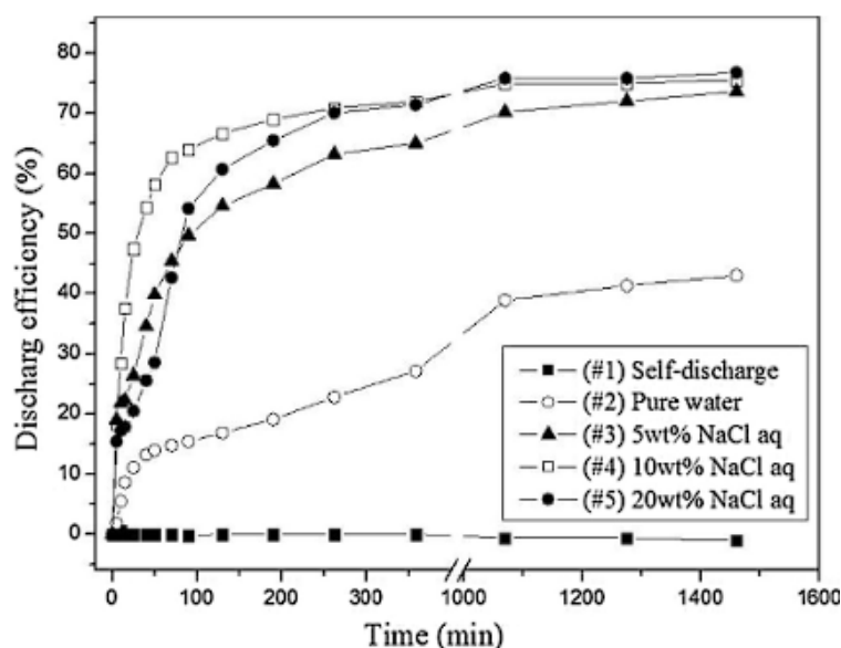
Figure 5.2. Discharge efficiency through time [389].
