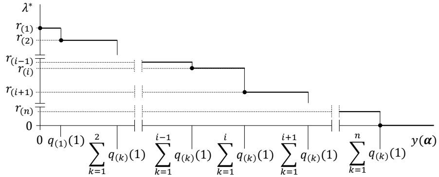
Figure 4.6: Optimal Lagrange multiplier \lambda^* vs. y(\alpha) .
