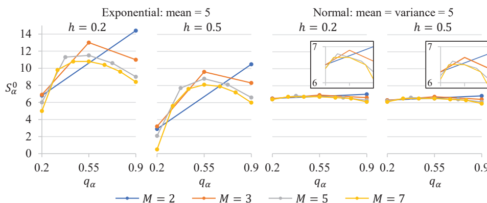
Figure 2.7: S_\alpha^0 vs. q_\alpha for b = 0.8 , r = 3.4 , the linear q_\alpha profile, two values of h , four values of M , and two demand distributions.
