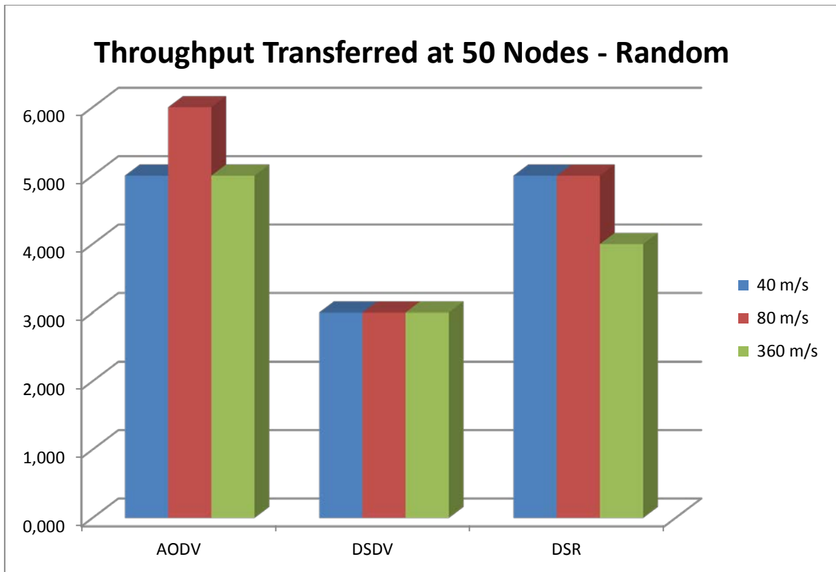
Figure 6.24 - Throughput Transferred at 50 Nodes – Random
