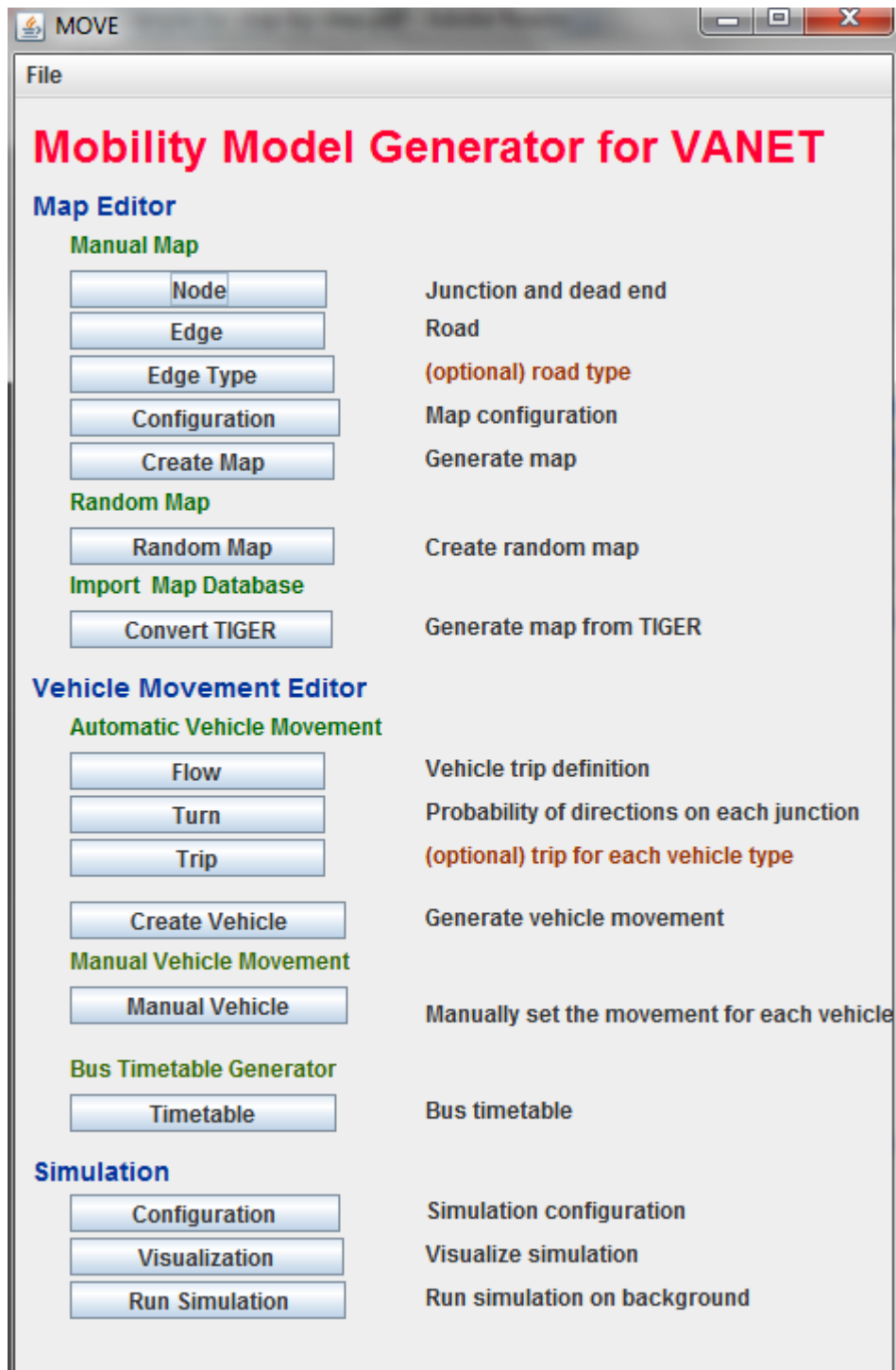
Figure 5.5.2 - Mobility Model
