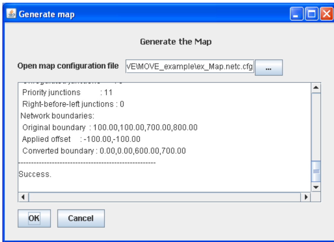
Figure 5.5.7 - Generate Map
