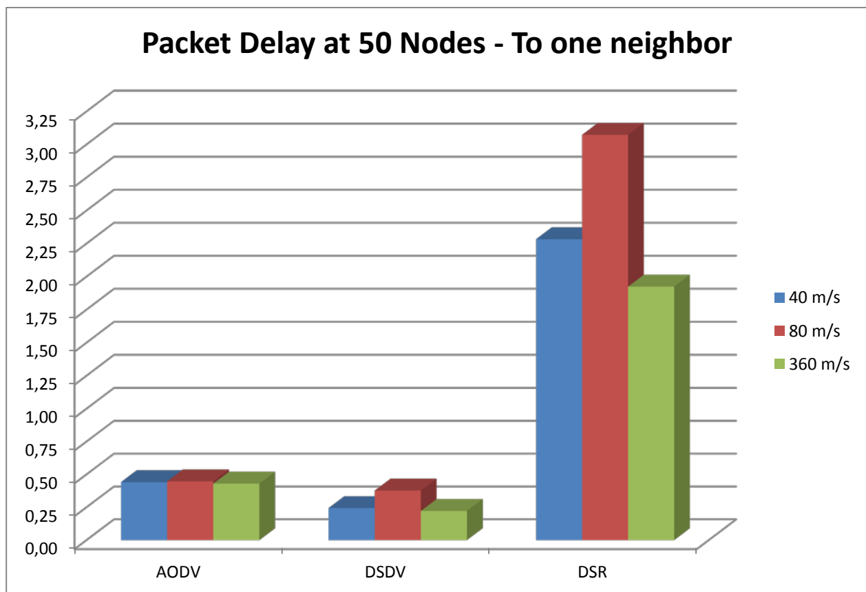
Figure 6.9 - Packet Delay at 50 Nodes – to one neighbor
