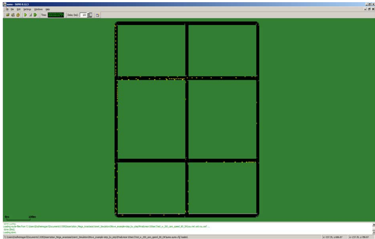
Figure 6.1 - Sumo map
