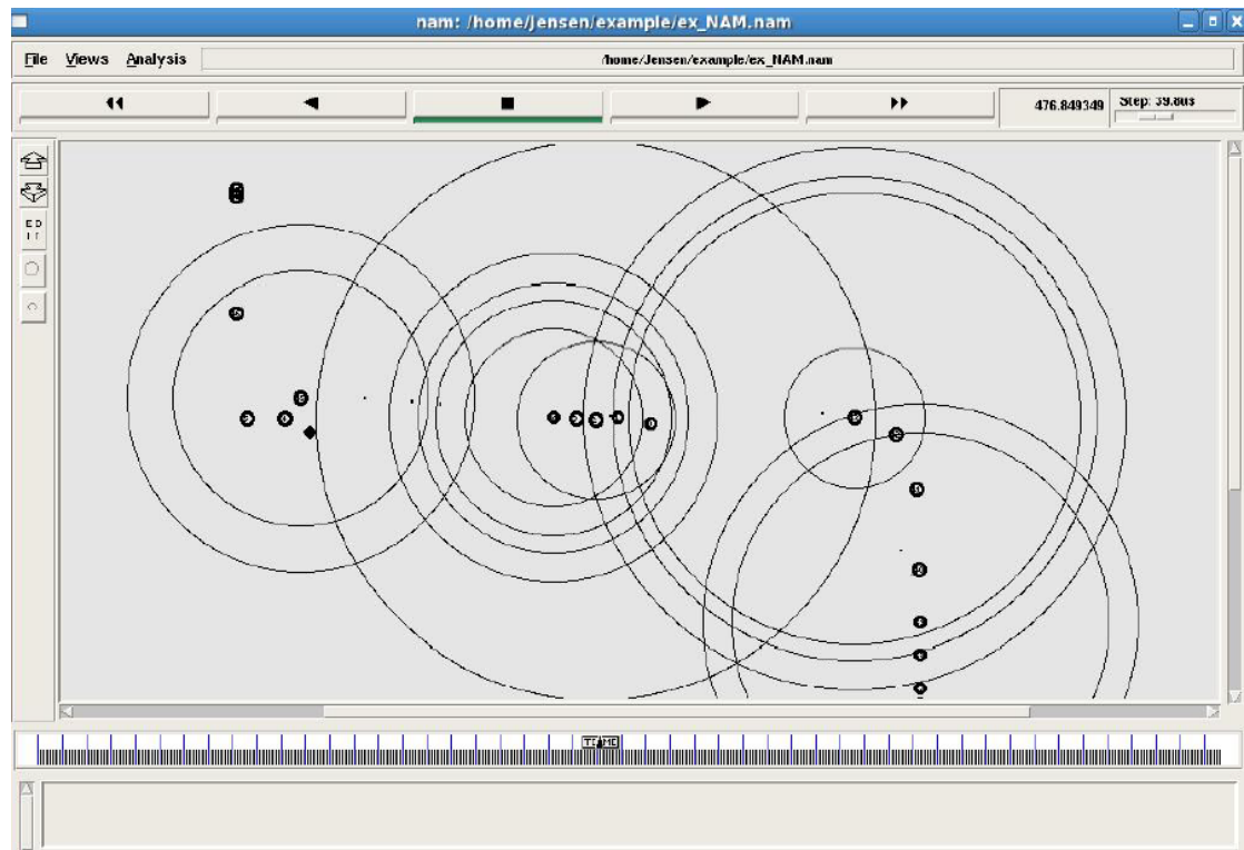
Figure 5.5.15 - NAM environment
