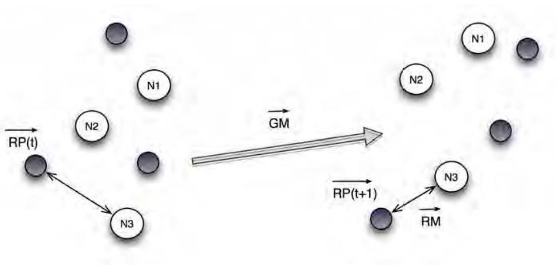
Figure 4.1.2.a - RPGM model Movements of three nodes according to the RPGM mobility model
