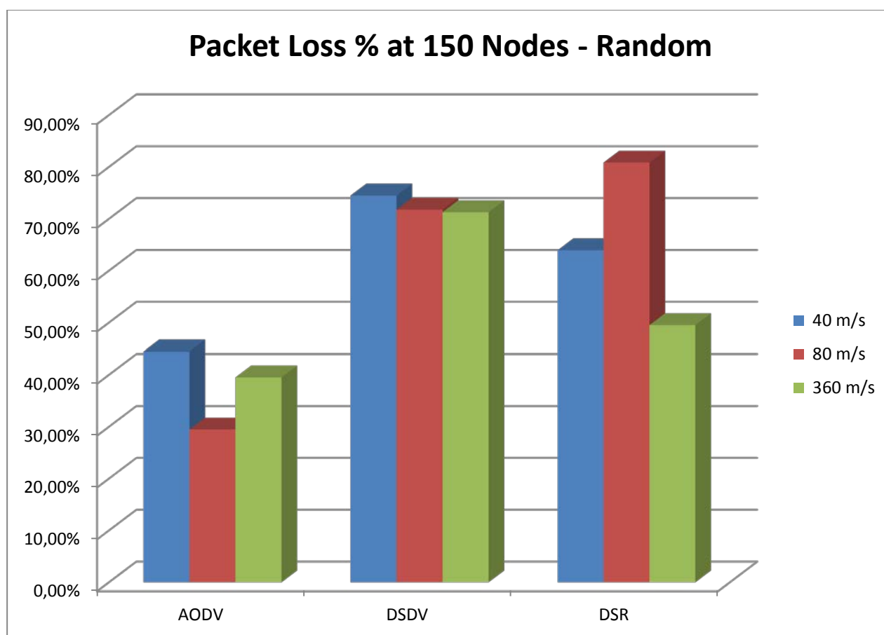
Figure 6.8 - Packet loss % at 150 Nodes – Random
