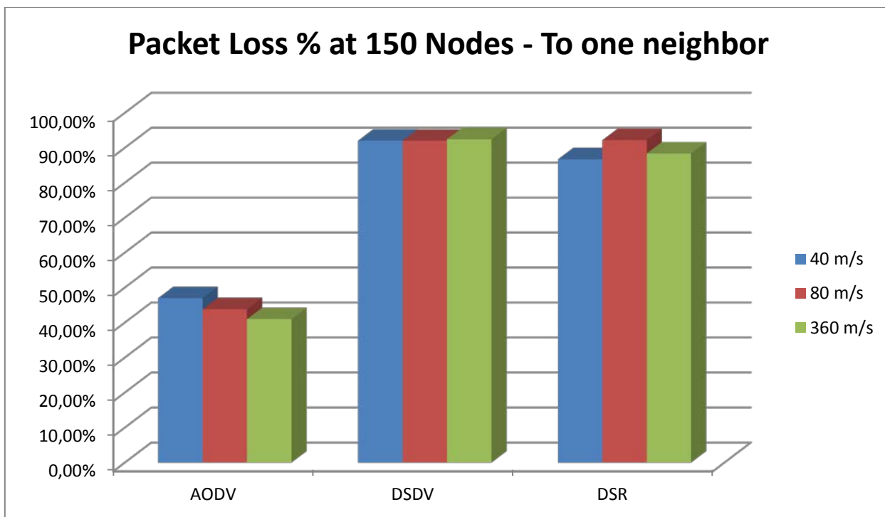
Figure 6.5 - Packet loss % at 150 Nodes – to one neighbor
