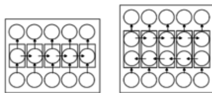
Figure 62 On the left, a typical RNN architecture. On the right, a BRNN architecture with two hidden layers [108]
