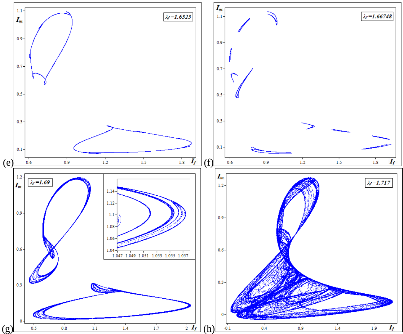
Figure 22 The phase plot ( I_f , I_m ) for \delta = 2.65 as \lambda_f increases in the interval \lambda_f \in [1.59, 1.72] . (a) Solutions converge to attracting 2-period cycle ( \lambda_f = 1.5743 ), (b) The birth of two closed invariant curves ( \lambda_f = 1.5916 ), (c) The invariant curves become kinked ( \lambda_f = 1.6375 ), (d) The invariant curves split in a 64-period cycle ( \lambda_f = 1.6446 ), (e) The invariant curves reappear slightly deformed ( \lambda_f = 1.6525 ), (f) Invariant curves break into a 10-period motion ( \lambda_f = 1.66748 ), (g) Invariant curves evolve into contiguous bands ( \lambda_f = 1.69 ), (h) Solutions converge to a strange attractor ( \lambda_f = 1.717 ).
