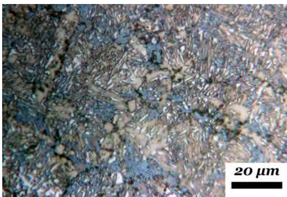
Figure 4.7: Metallography of heat treatment C picture 2
