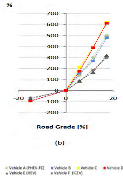
Figure 22: Energy consumption variation, Cascais-Lisboa driving cycle (34.2km) [Figure 5(b), (Ribau, Silva, & Farias, 2010)].
