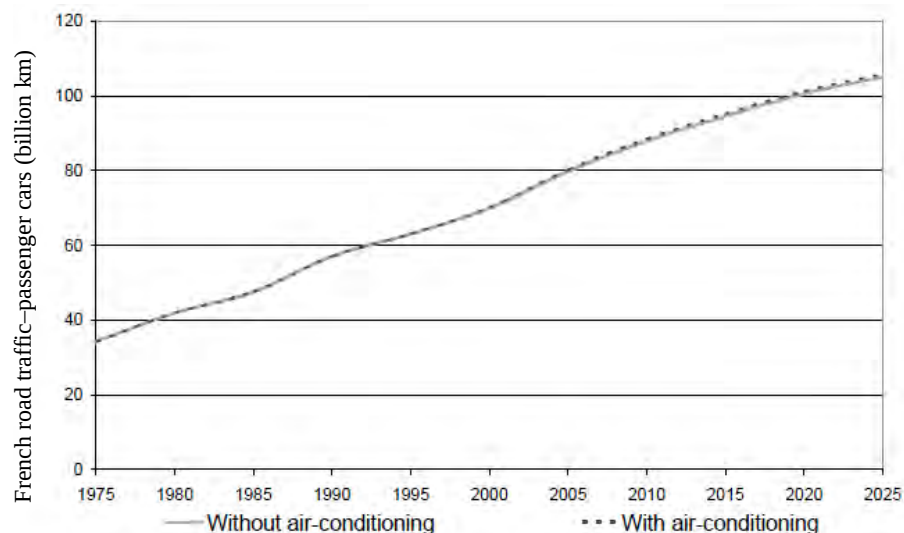
Figure 31: Influence of air-conditioning on passenger car CO 2 emissions (10 6 t) (Hugrel & Joumard, September 17-19, 2001).
