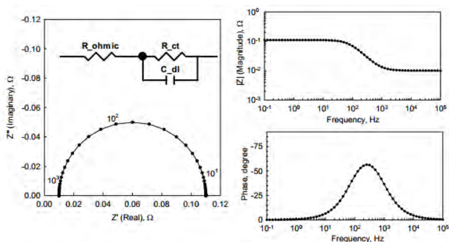
Figure 3.14: Impedance plots for the indicated simple RC circuit where R_{ohmic} = 0.01 \Omega , R_{ct} = 0.1 \Omega and C_{dl} = 0.02 \text{ F} .
