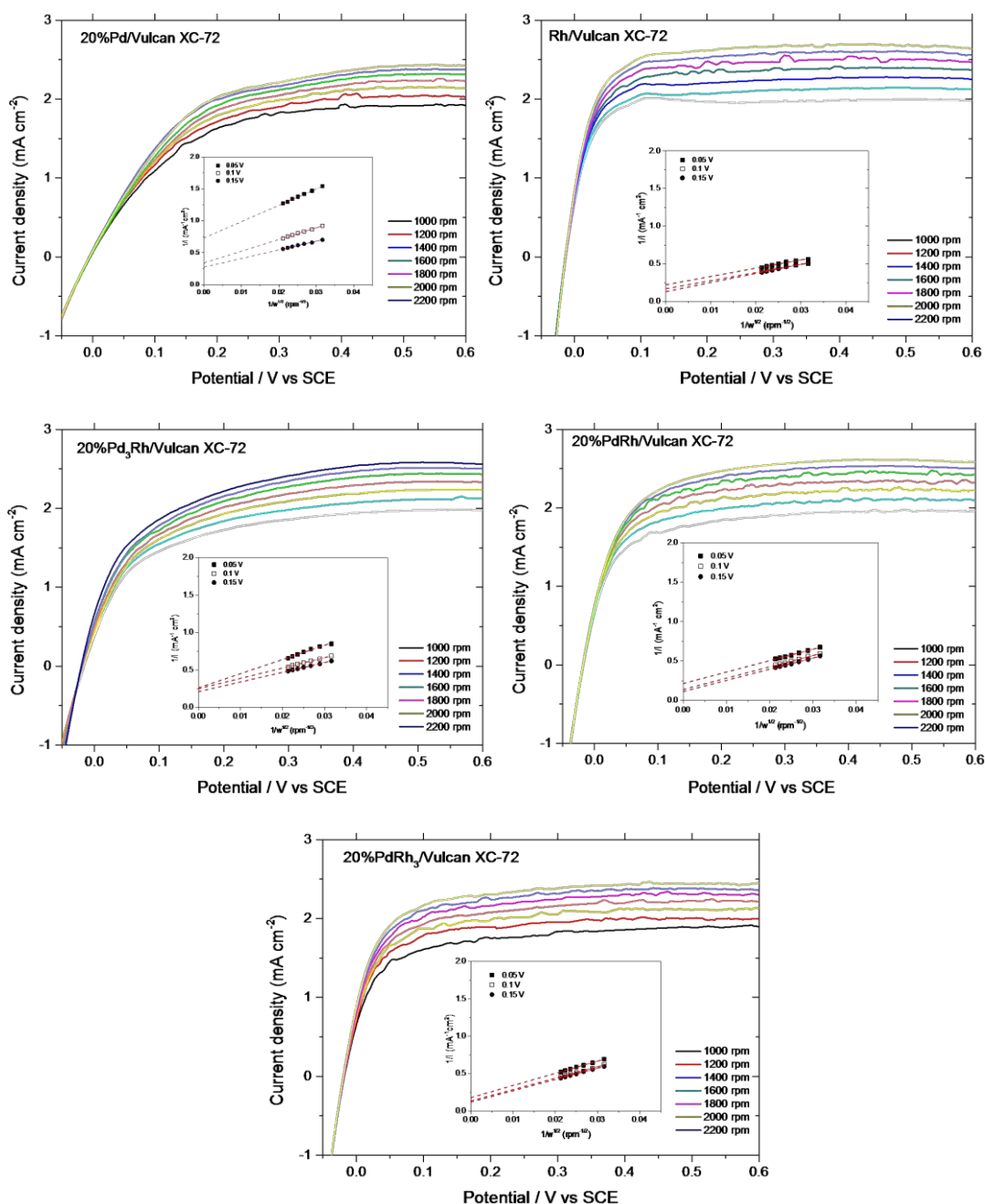
Figure 4.4: RDE curves in \text{H}_2 -saturated 0.5 M \text{H}_2\text{SO}_4 , scan rate: 5 \text{ mV s}^{-1} . Insets: Koutecky-Levich plots. The insets are the corresponding Koutecky-Levich plots for the hydrogen oxidation reaction.
