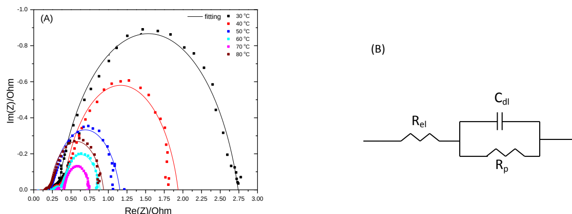
Figure 7.8: MEA impedance plots with H 2 /O 2 feeding (H 2 : 80 mLmin -1 , O 2 : 40 mLmin -1 ), from 1 mHz– 100 kHz . Ac:10mV at 0.6 V at different temperatures of 30-80°C, at atmospheric pressure (A), Nyquist equivalent circuit (B).
