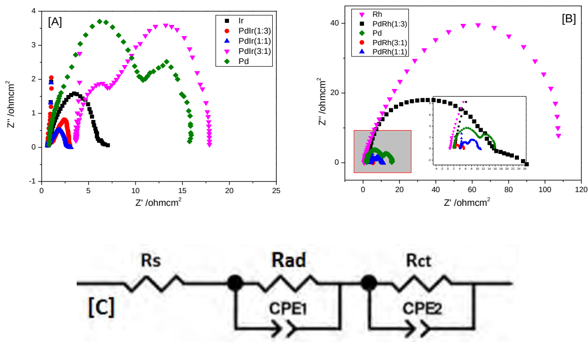
Figure 8.10: Nyquist plots for different alloys at 0.35 V in 0.5M \text{H}_2\text{SO}_4 .
