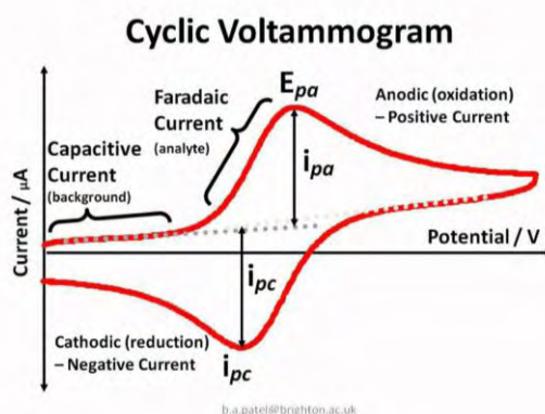
Figure 3.4: A typical cyclic voltammogram for a reversible reaction.
