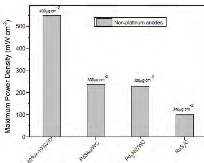
Figure 2.6: Maximum Power Density (mWcm -2 ) over different Pt-free anodes.
