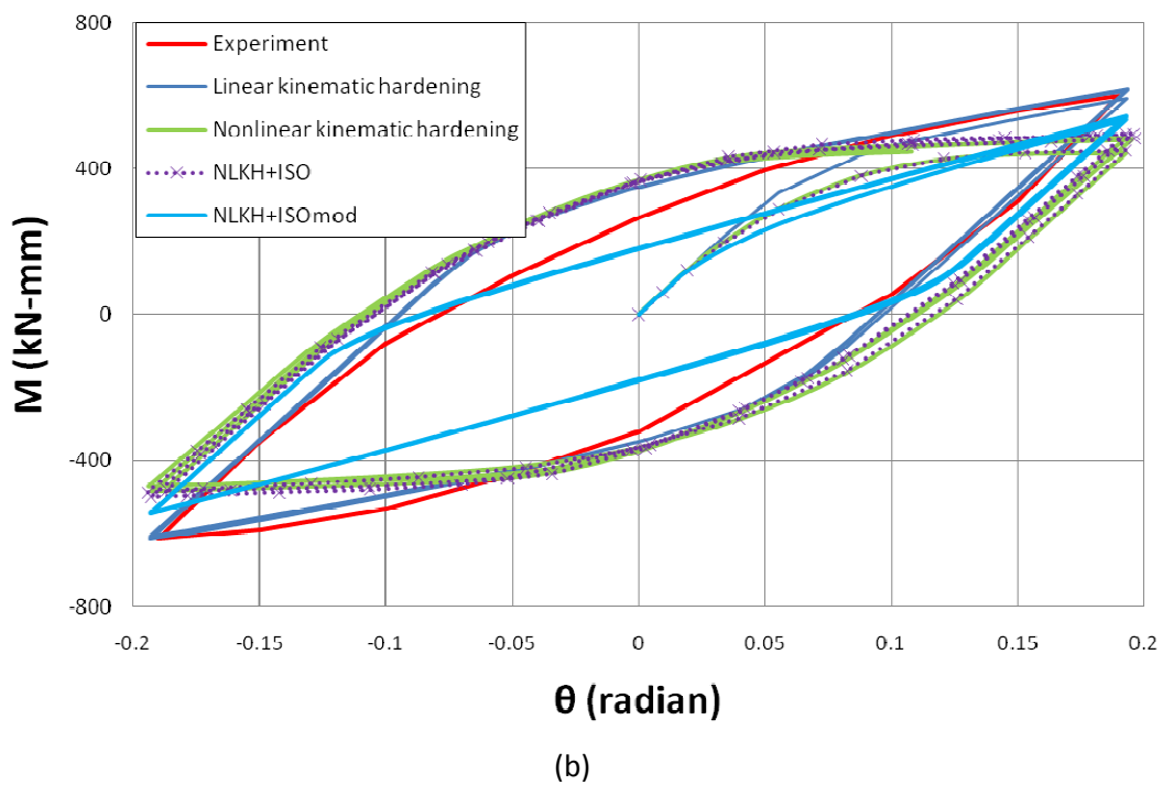
Figure 3.14: Moment rotation diagrams. (a) Applied rotation \theta_c = 0.0924 \text{ rad} (b) Applied rotation \theta_c = 0.1930 \text{ rad}
