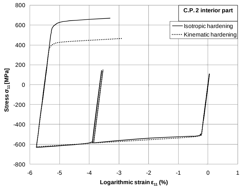
Figure 4.16: The stress strain path for the C.P.2: (a) outer surface, (b) inner surface.
