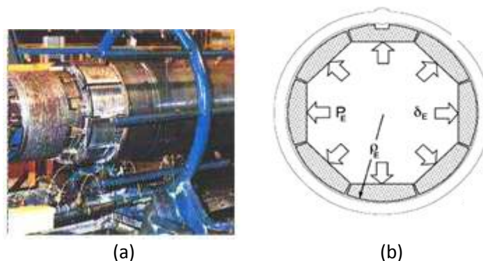
Figure 4.5: Pipe expansion
