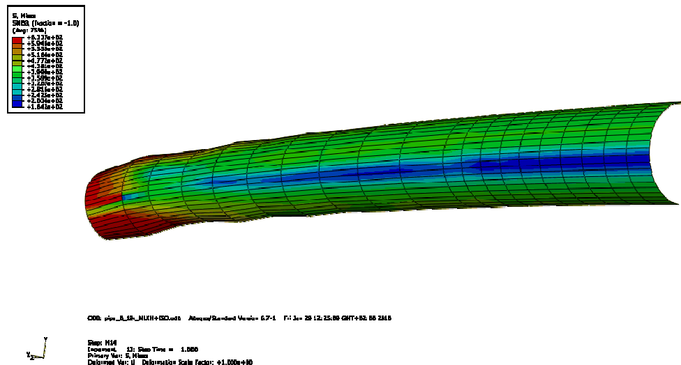
Figure 3.15: Localization of plastic deformations on the deformed geometry of the pipe after a few loading cycles.
