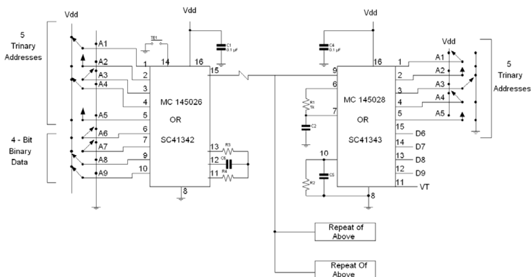
Figure 4. Typical Application
